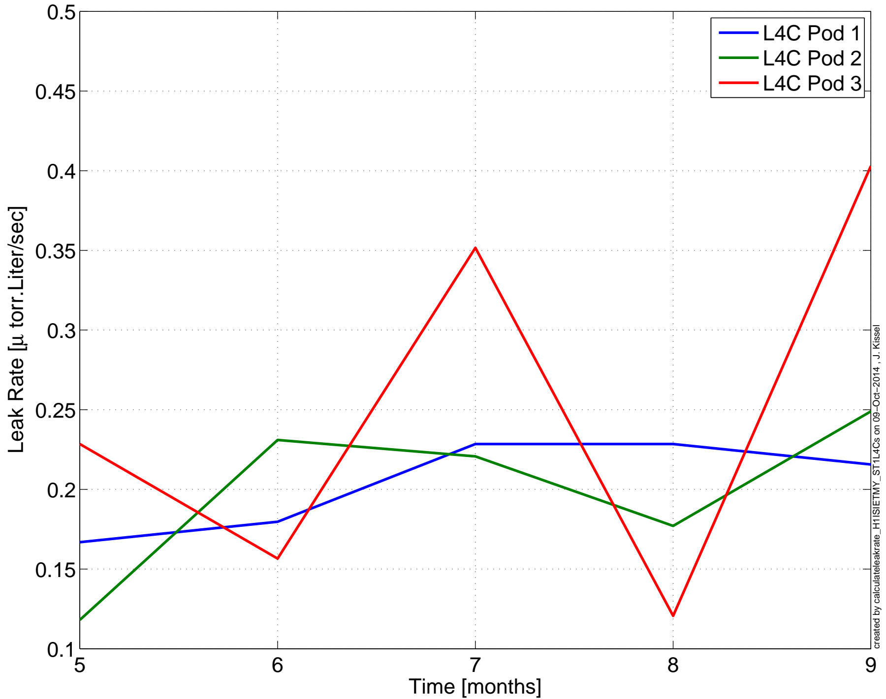
2014–May to 2014–Oct H1 ISI ETMY, L4C Pod Leak Rate Converted Absolute Pressure Sensor Readings
