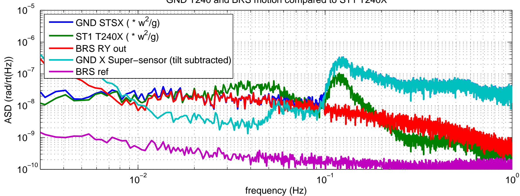
GND T240 and BRS motion compared to ST1 T240X
