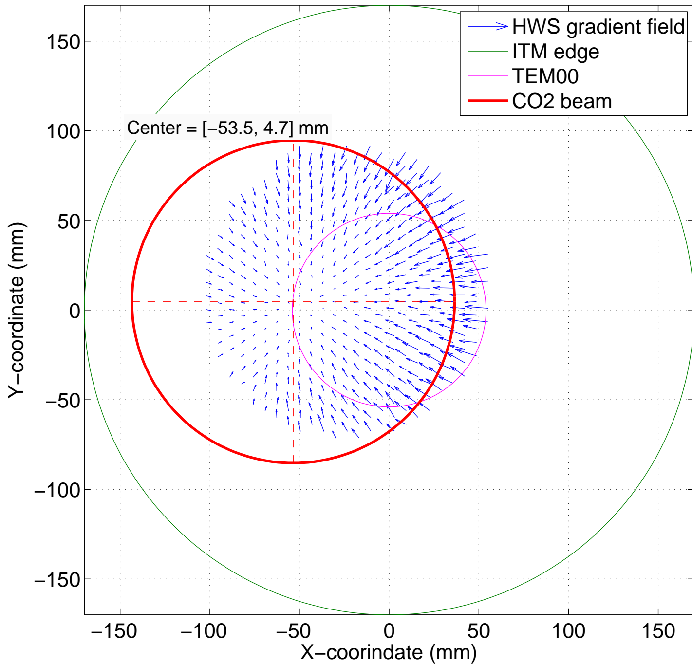
H1-ITMX CO2 thermal lens at t = 3920s from heating start time, measured by HWS
