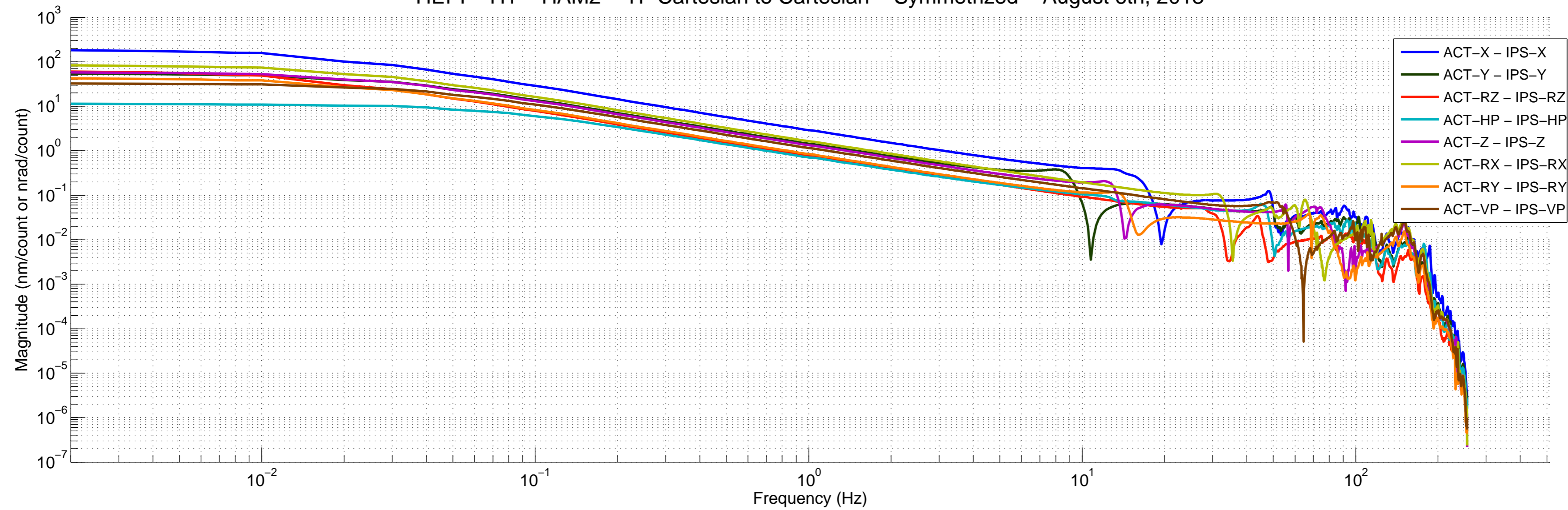
HEPI – H1 – HAM2 – TF Cartesian to Cartesian – Symmetrized – August 6th, 2013
