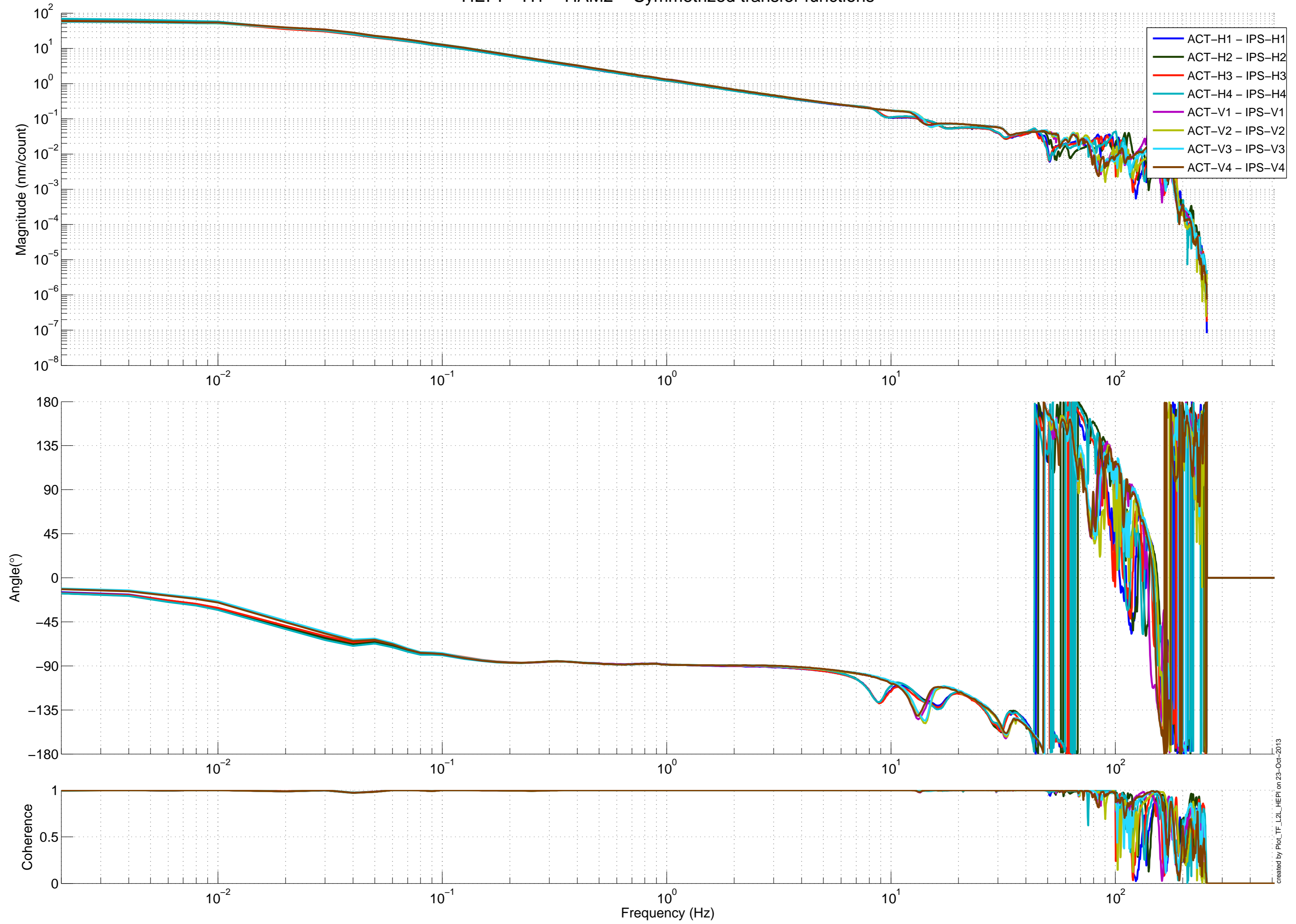
HEPI - H1 - HAM2 - Symmetrized transfer functions
