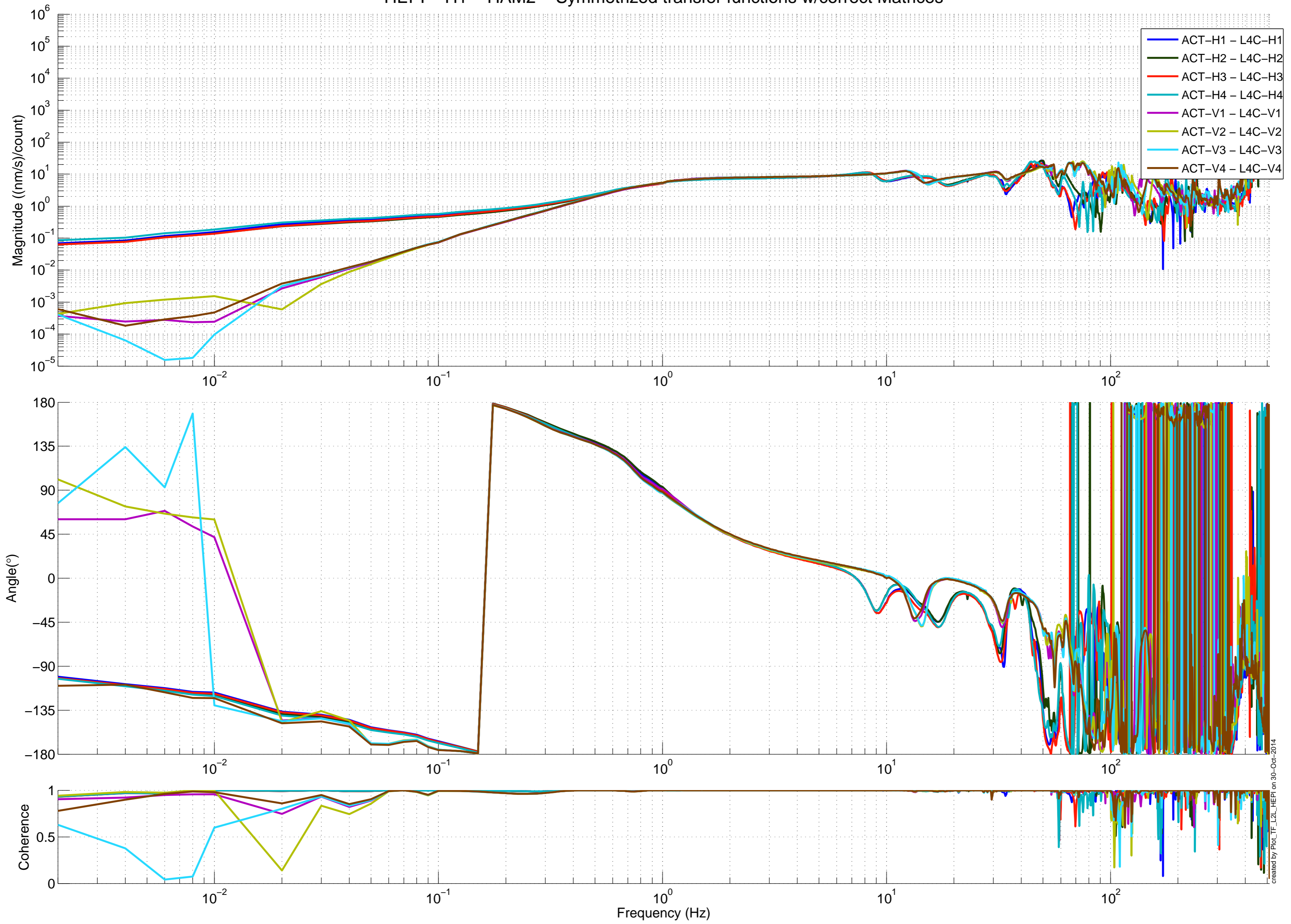
HEPI - H1 - HAM2 - Symmetrized transfer functions w/correct Matrices
