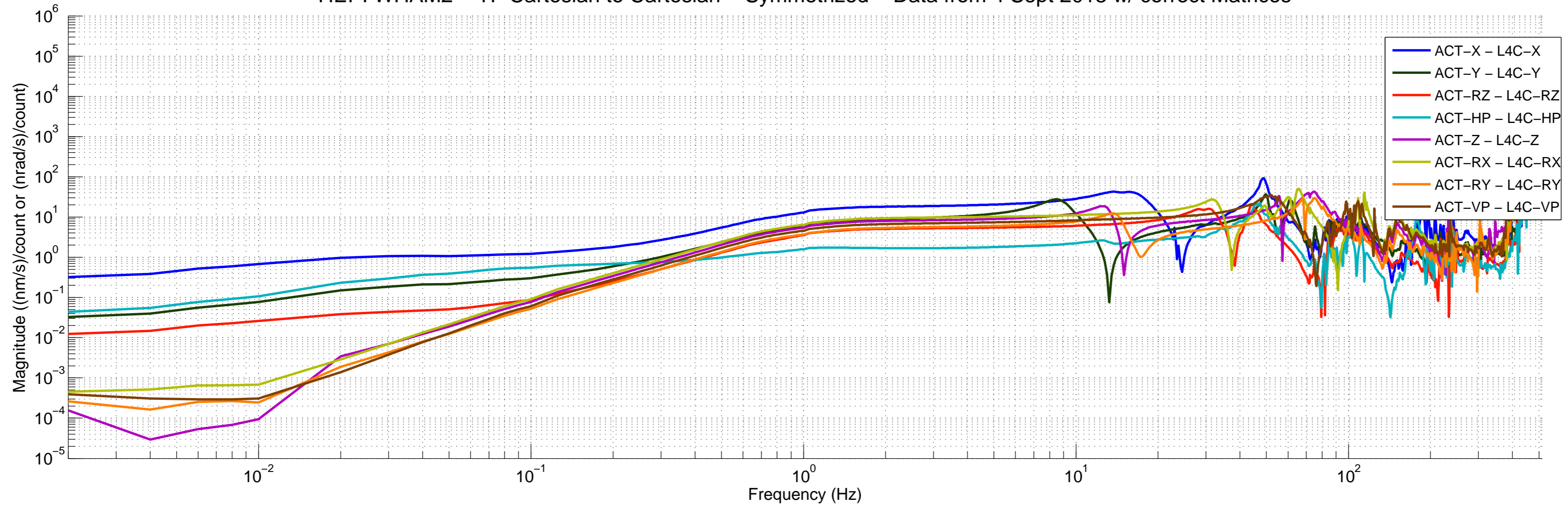
HEPI WHAM2 – TF Cartesian to Cartesian – Symmetrized – Data from 4 Sept 2013 w/ correct Matrices
