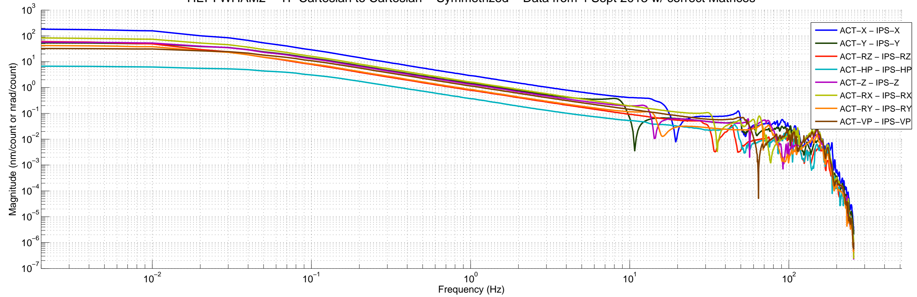
HEPI WHAM2 – TF Cartesian to Cartesian – Symmetrized – Data from 4 Sept 2013 w/ correct Matrices
