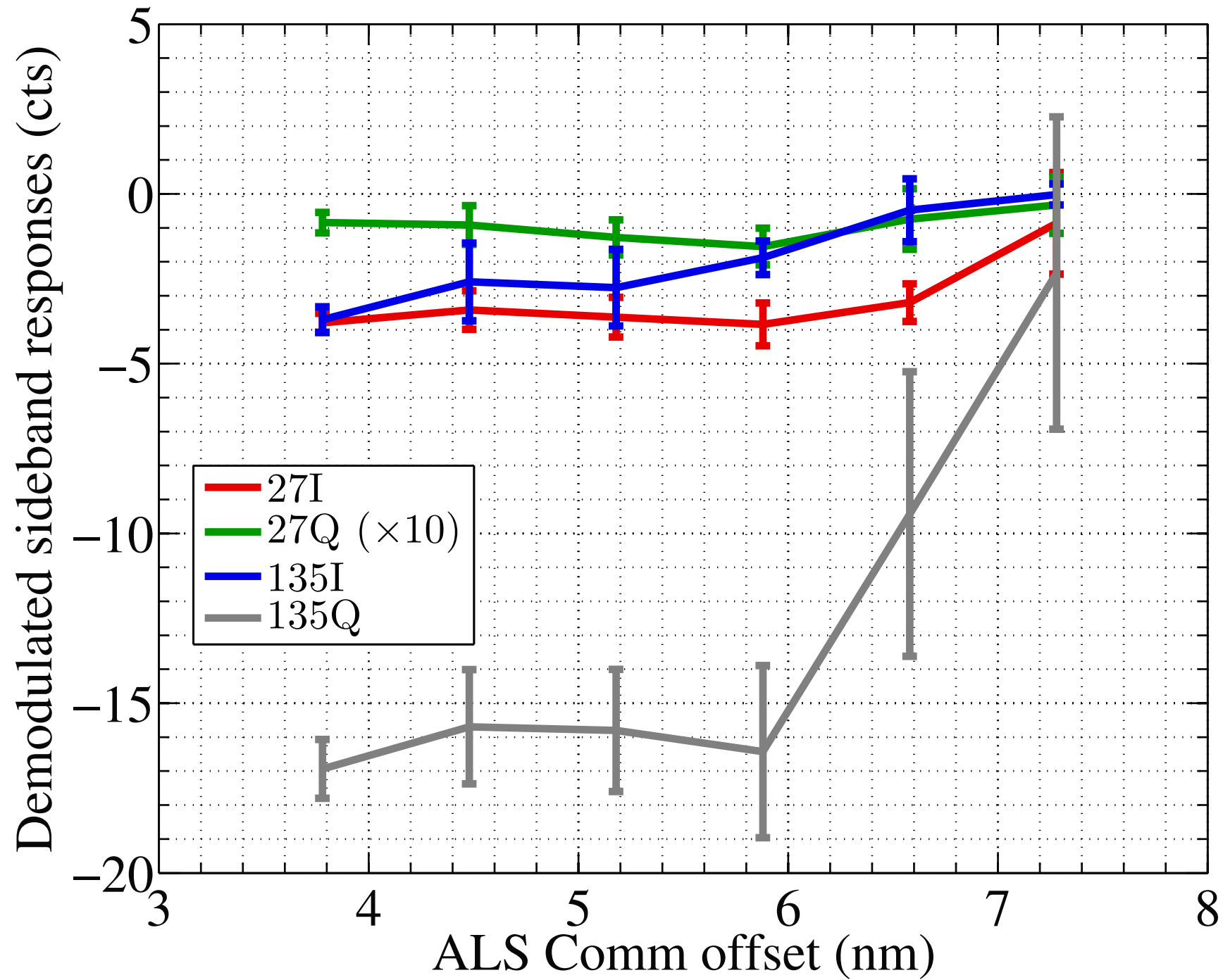
DRMI 3f sensing matrix, SR2
