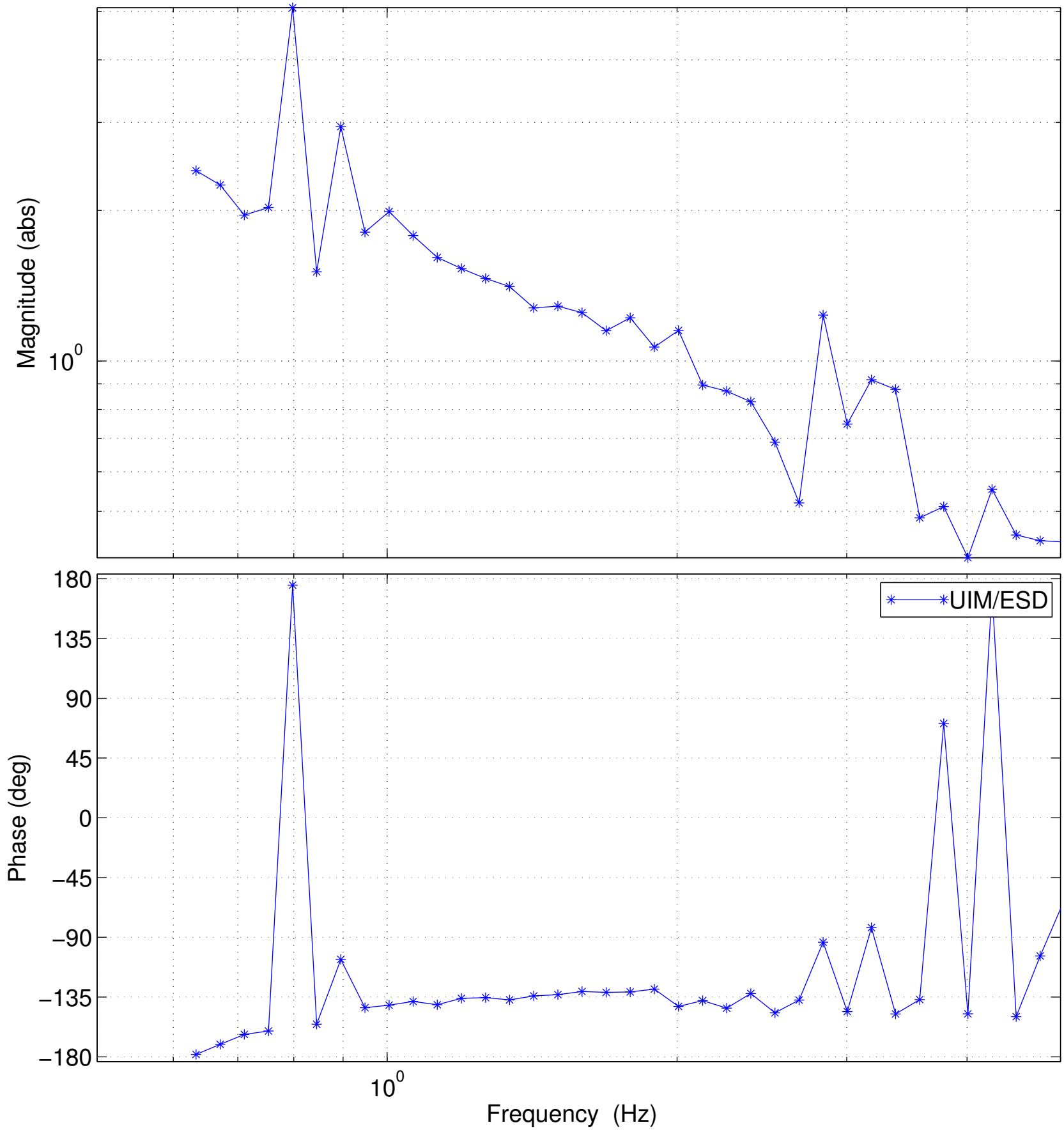
Bode Diagram
