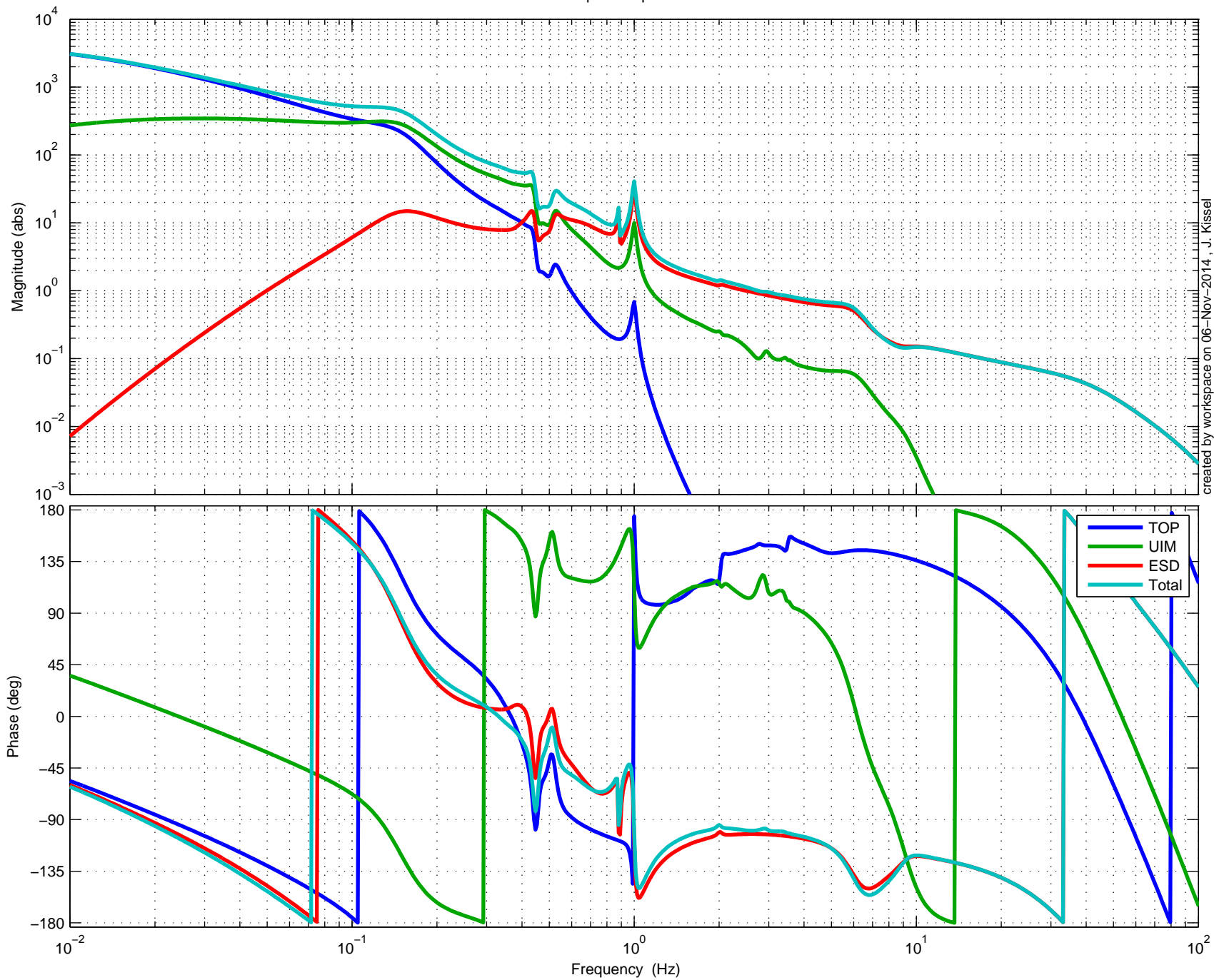
SISO DARM Open Loop Gain Breakdown
