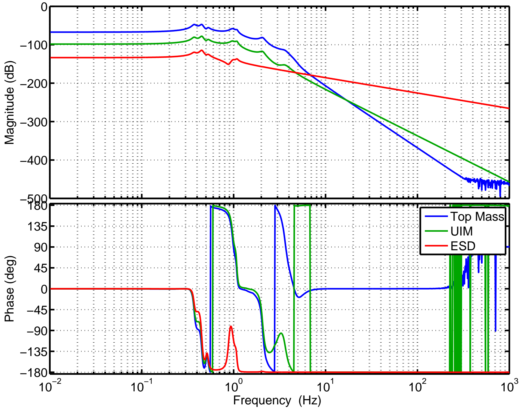
QUAD Plant Transfer Functions
