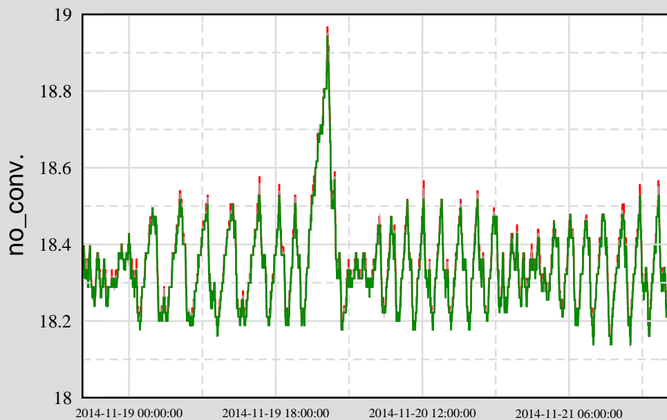
Ch 1: H0:FMC-EX_VEA_AVTEMP_DEGC
