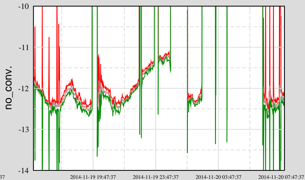
Ch 3: H1:SUS-ETMX_L3_OPLEV_YAW_OUT16
