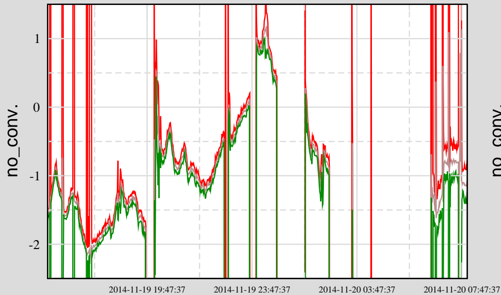
Ch 2: H1:SUS-ETMX_L3_OPLEV_PIT_OUT16
