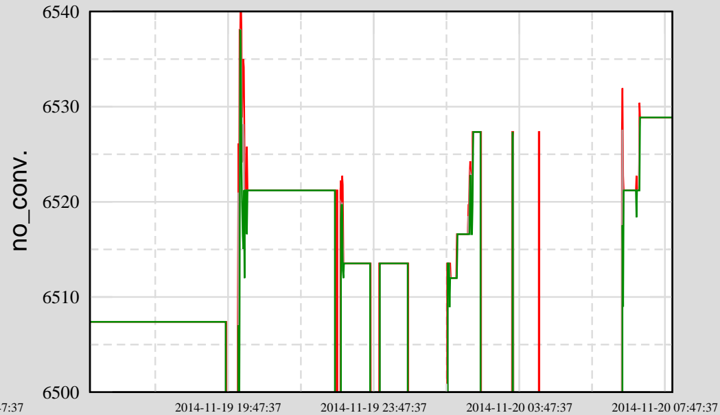
Ch 4: H1:SUS-ETMX_M0_OPTICALIGN_P_OUTPUT
