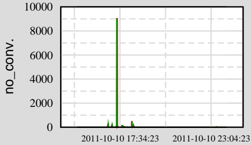
Ch 1: H0:PEM-LVEA_DST12_5
