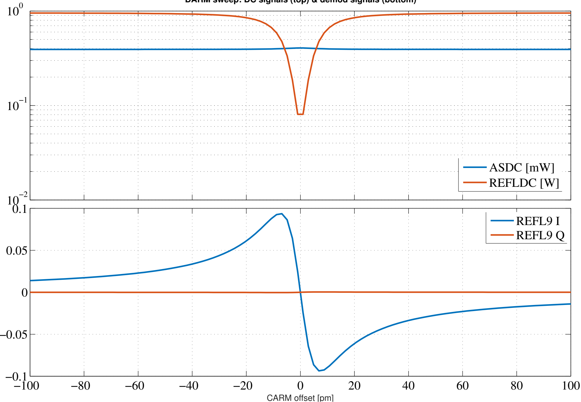
DARM sweep: DC signals (top) & demod signals (bottom)
