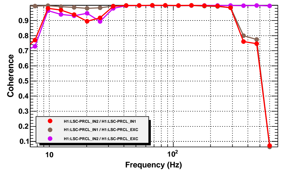
T0=04/12/2014 03:44:01.200073 Avg=8
