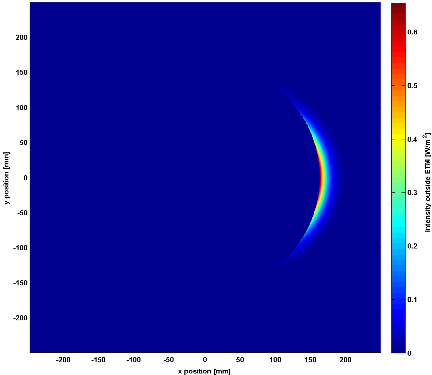
Intensity outside ETM coating for 6cm offset beam
