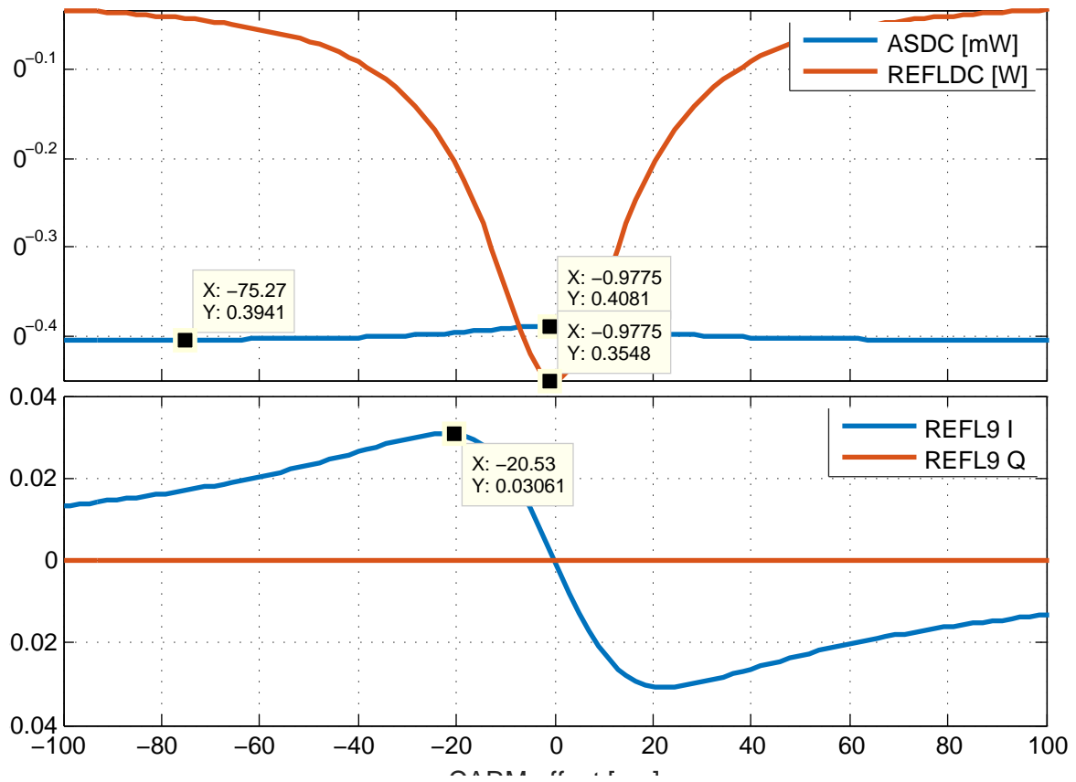
DARM sweep: DC signals (top) & demod signals (bottom)
