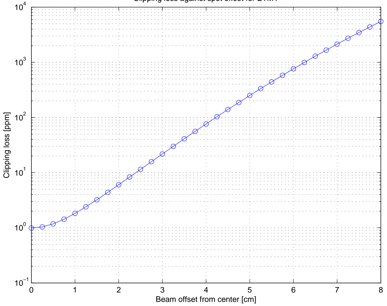
Clipping loss against spot offset for ETMY
