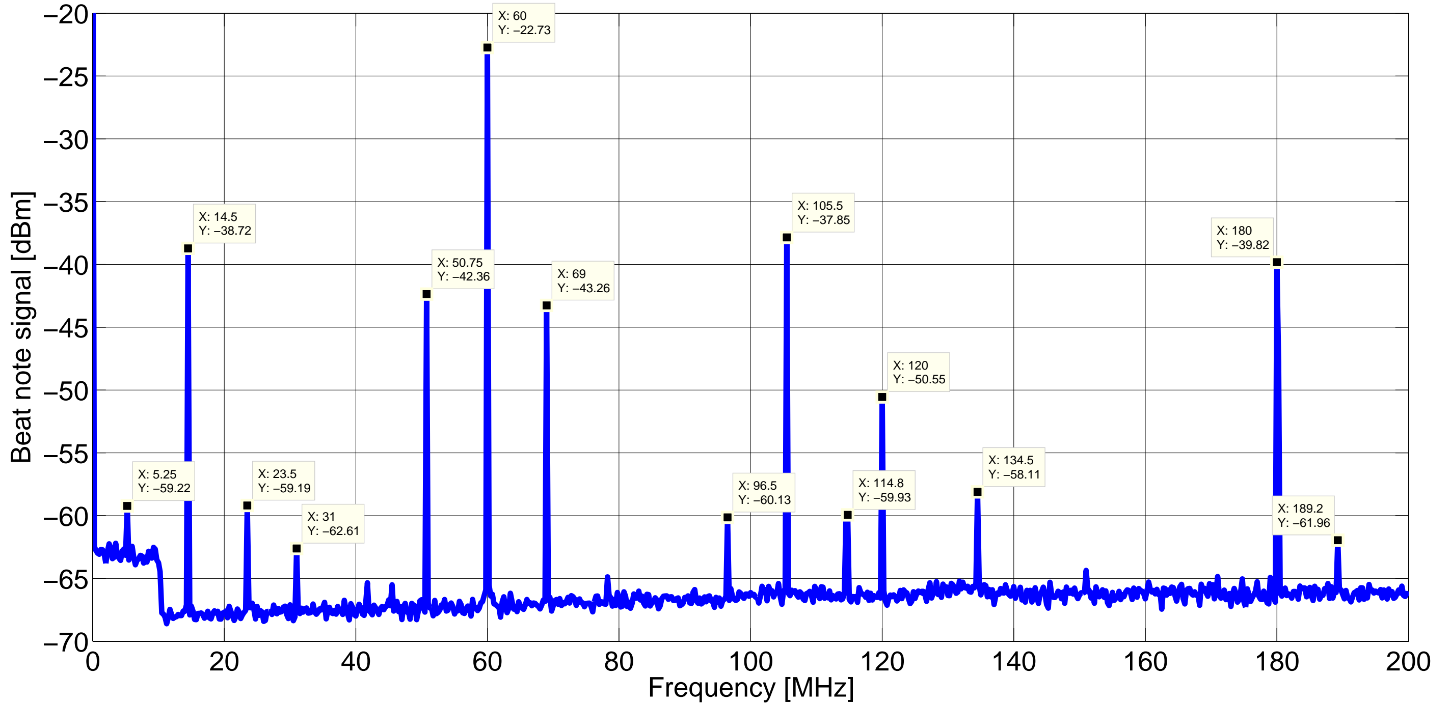
RFPD output spectrum with aux laser phase locked to PSL with 60MHz offset
