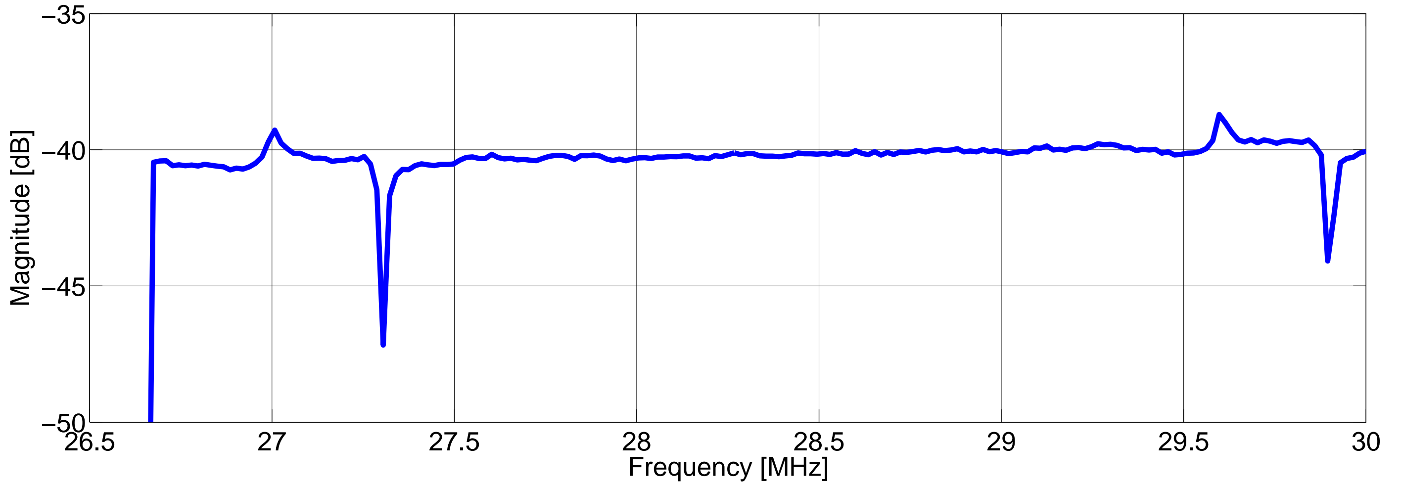
27.3MHz to 29.9MHz full FSR aux sweep TF
