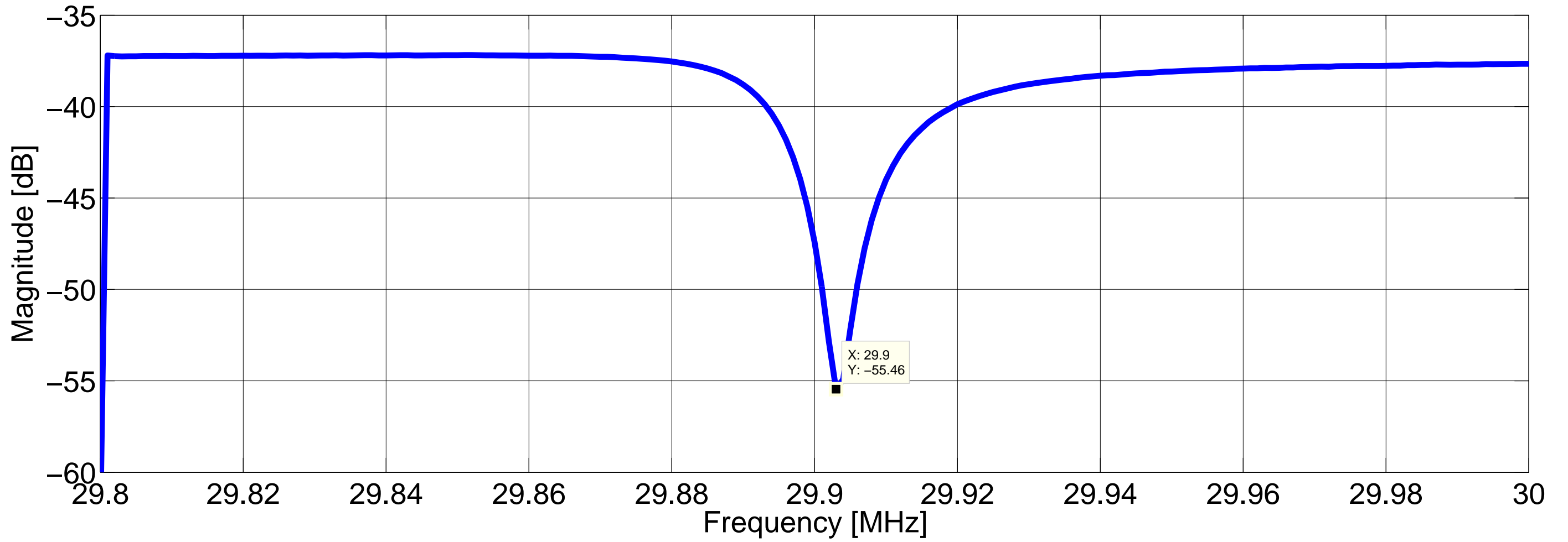
29.9MHz FSR aux sweep TF
