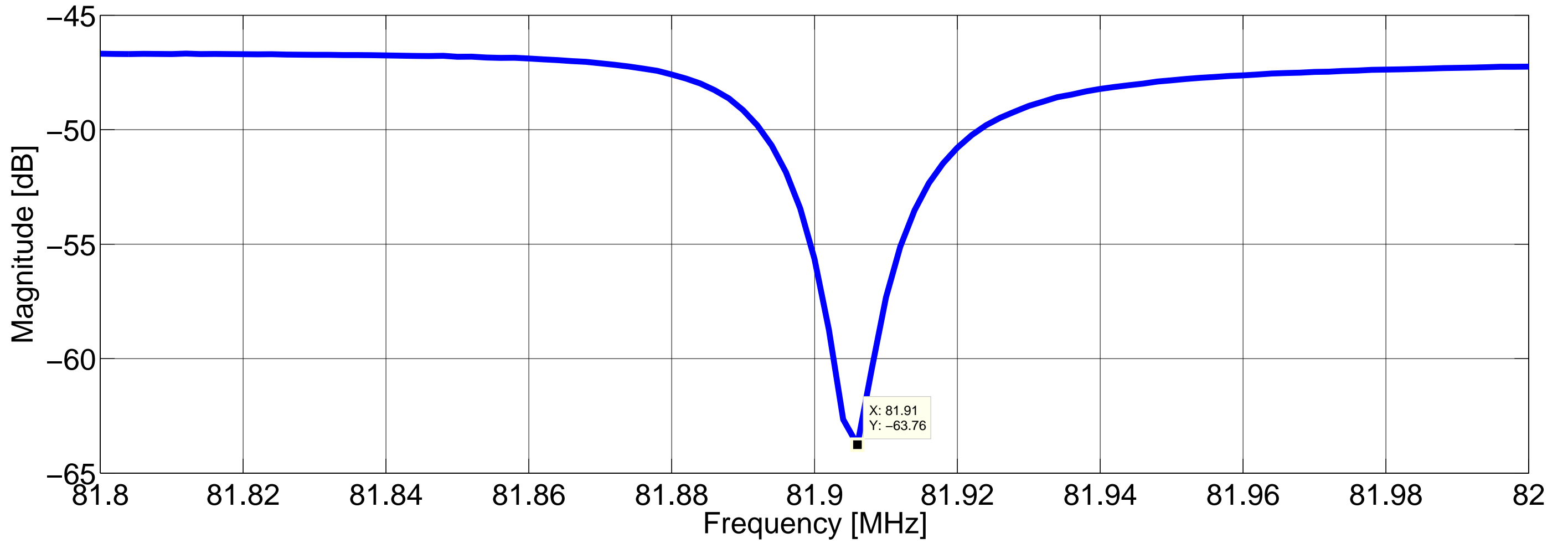
81.9MHz FSR aux sweep TF
