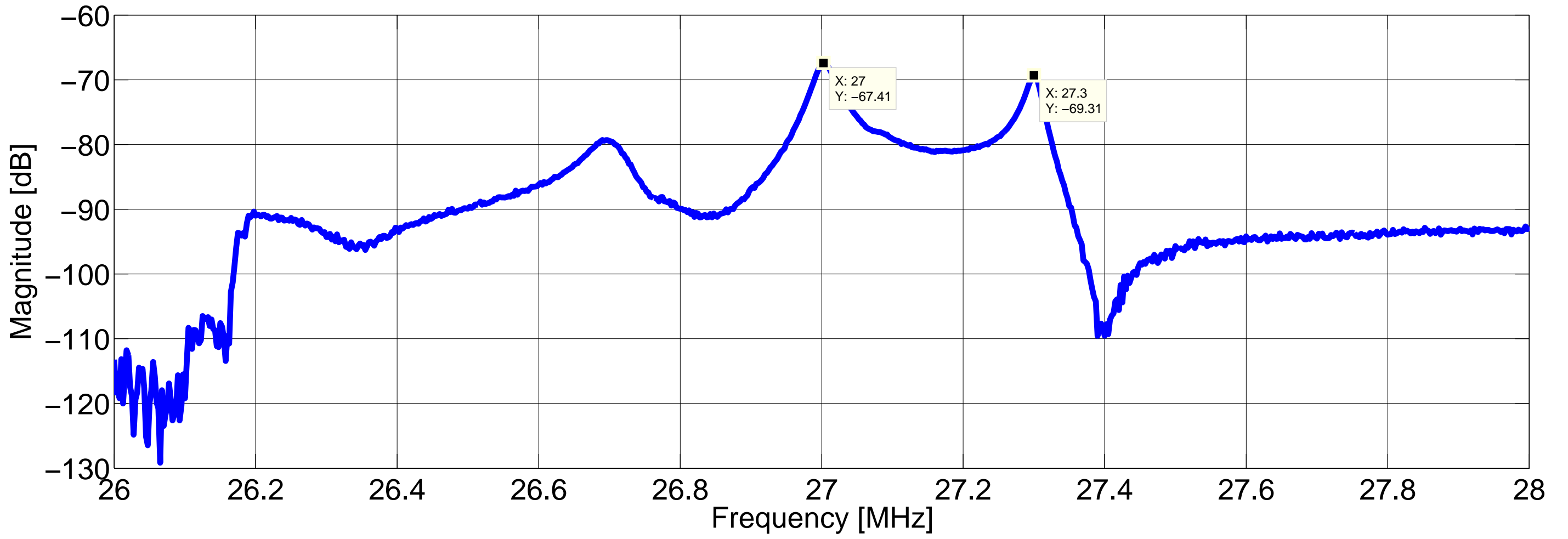
PRC higher order mode scan
