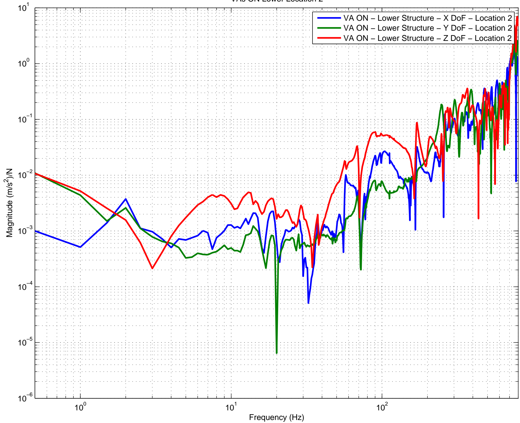
Vibration Absorbers Tap Test H2 FMY VAs ON Lower Location 2
