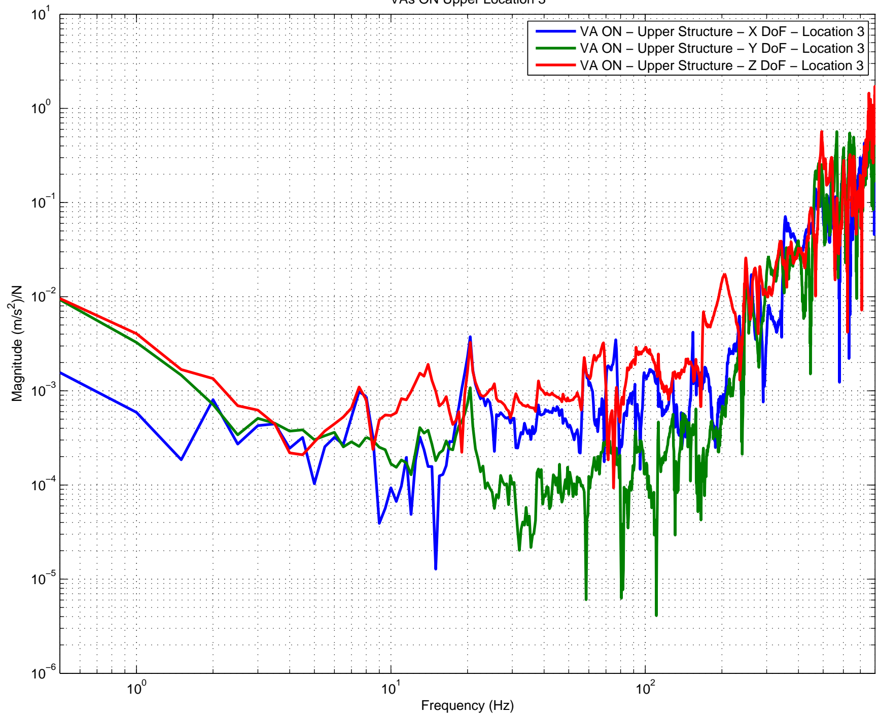
Vibration Absorbers Tap Test H2 FMY VAs ON Upper Location 3
