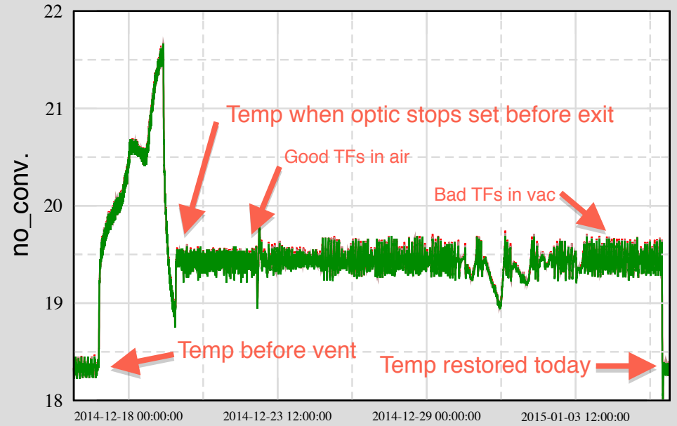
Ch 4: H0:FMC-EX_VEA_AVTEMP_DEGC
