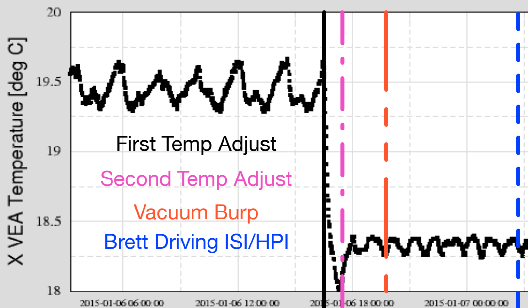
Ch 3: H0:FMC-EX_VEA_AVTEMP_DEGC
