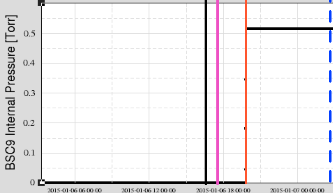
Ch 4: HVE-EX:X3_510ATORR
