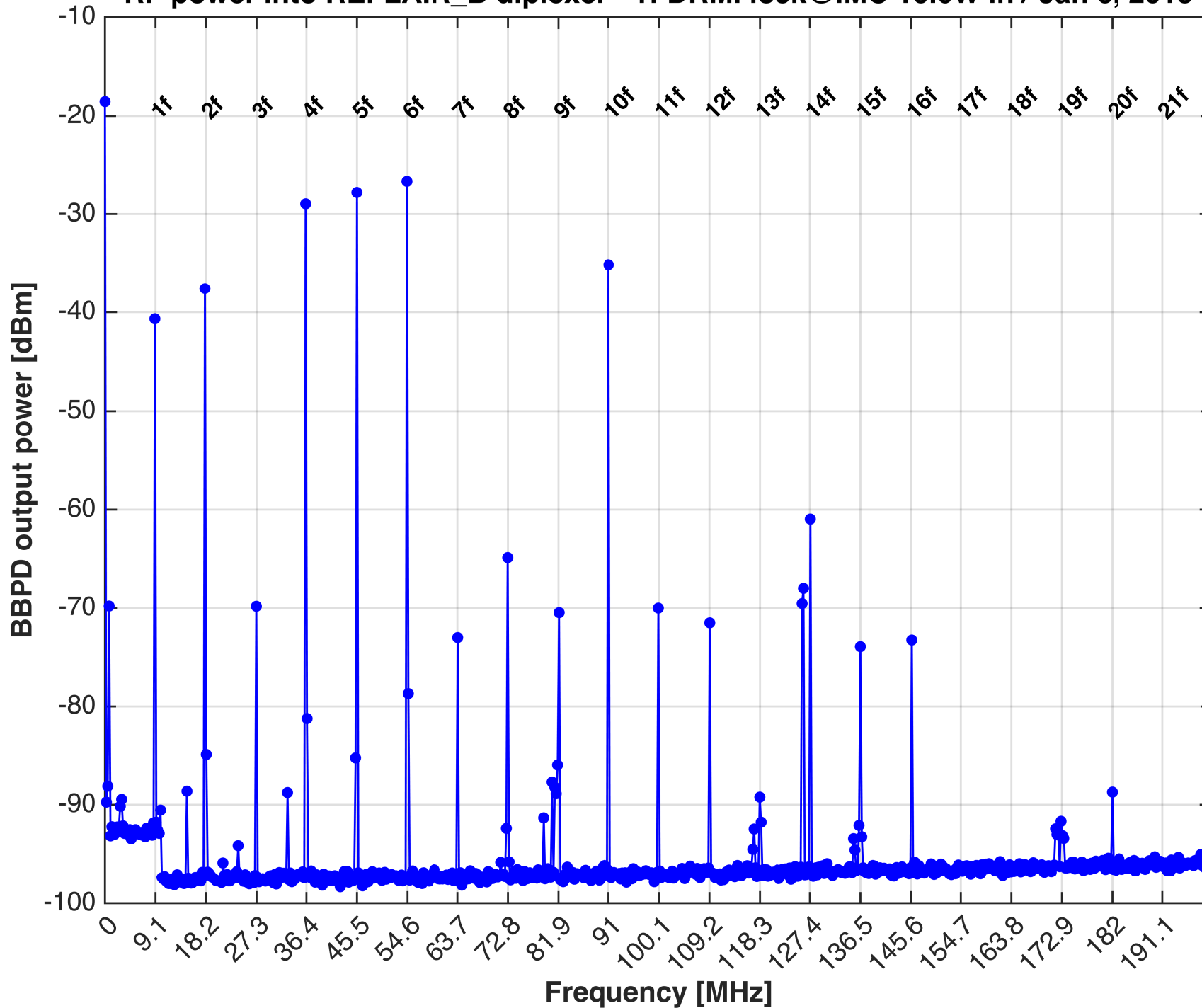
RF power into REFLAIR_B diplexer - 1f DRMI lock@IMC 10.6W in / Jan 6, 2015
