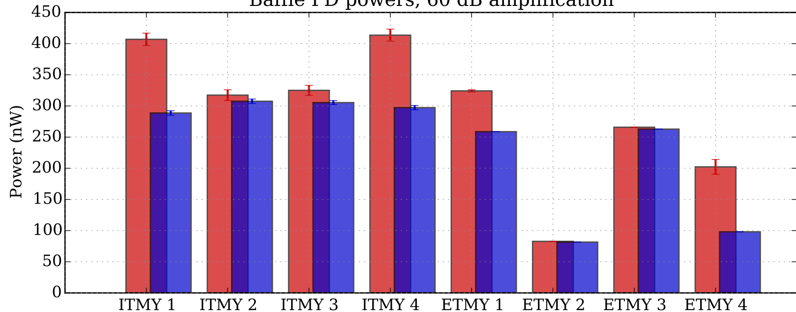
Baffle PD powers, 60 dB amplification
