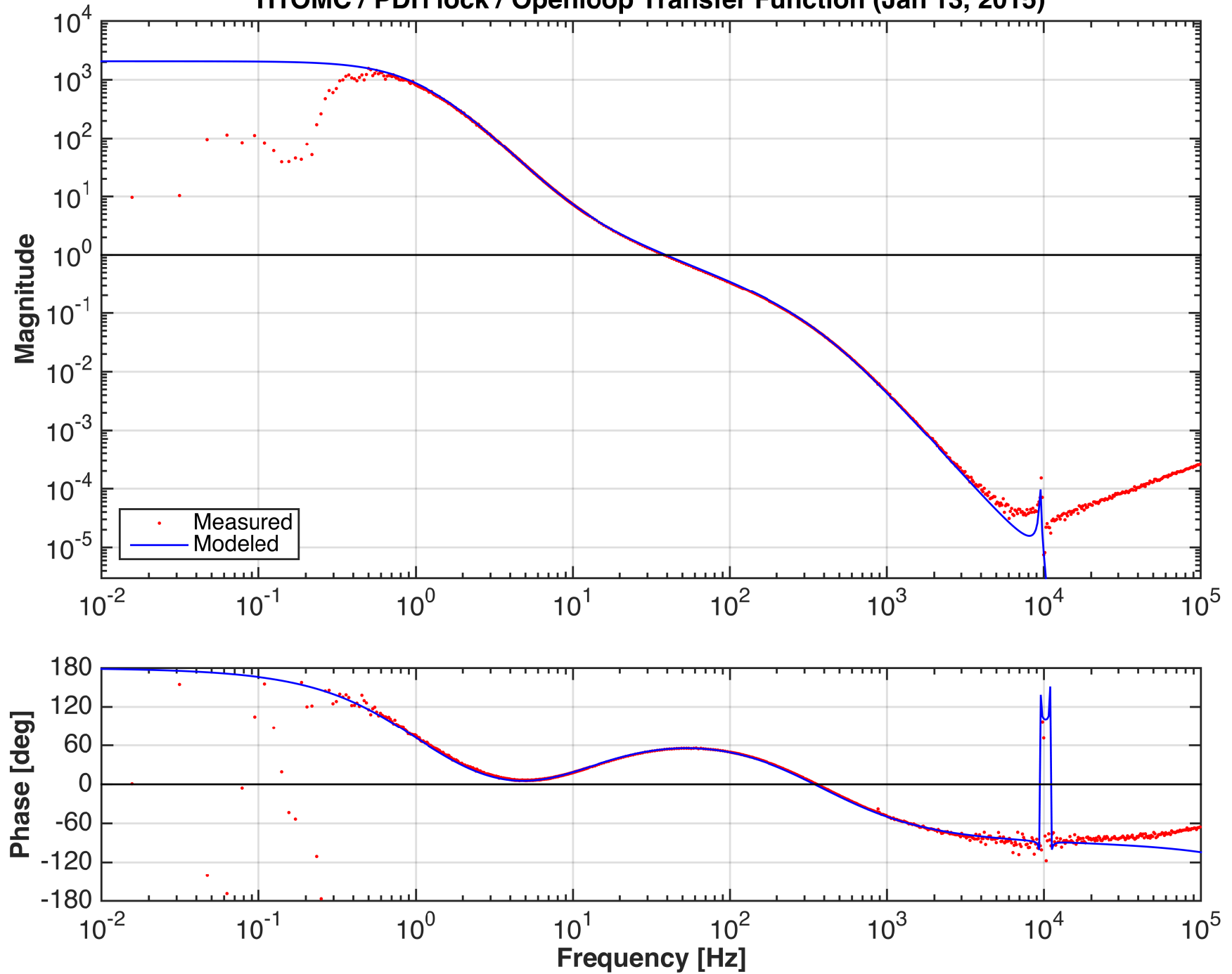
H1OMC / PDH lock / Openloop Transfer Function (Jan 13, 2015)
