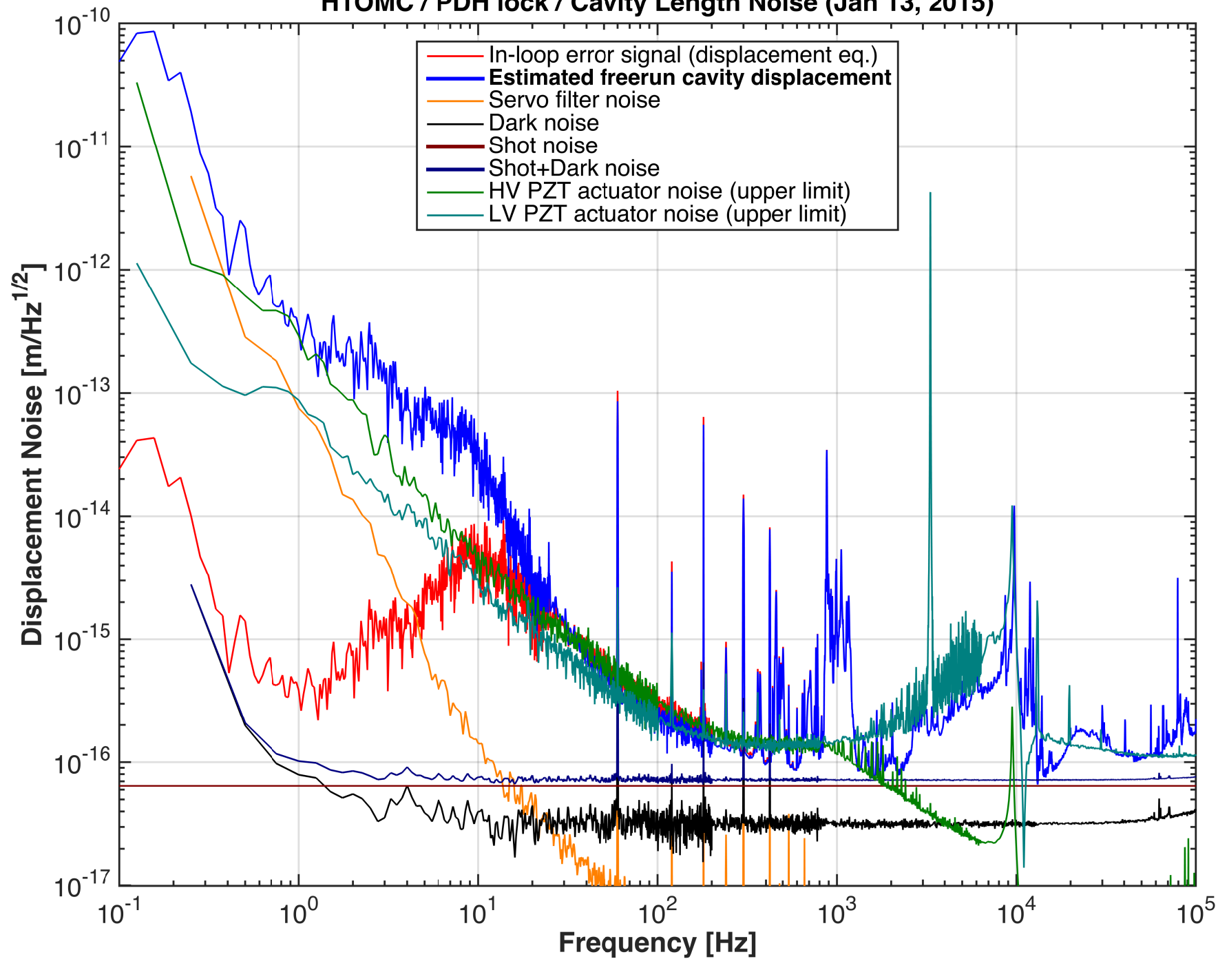
H1OMC / PDH lock / Cavity Length Noise (Jan 13, 2015)
