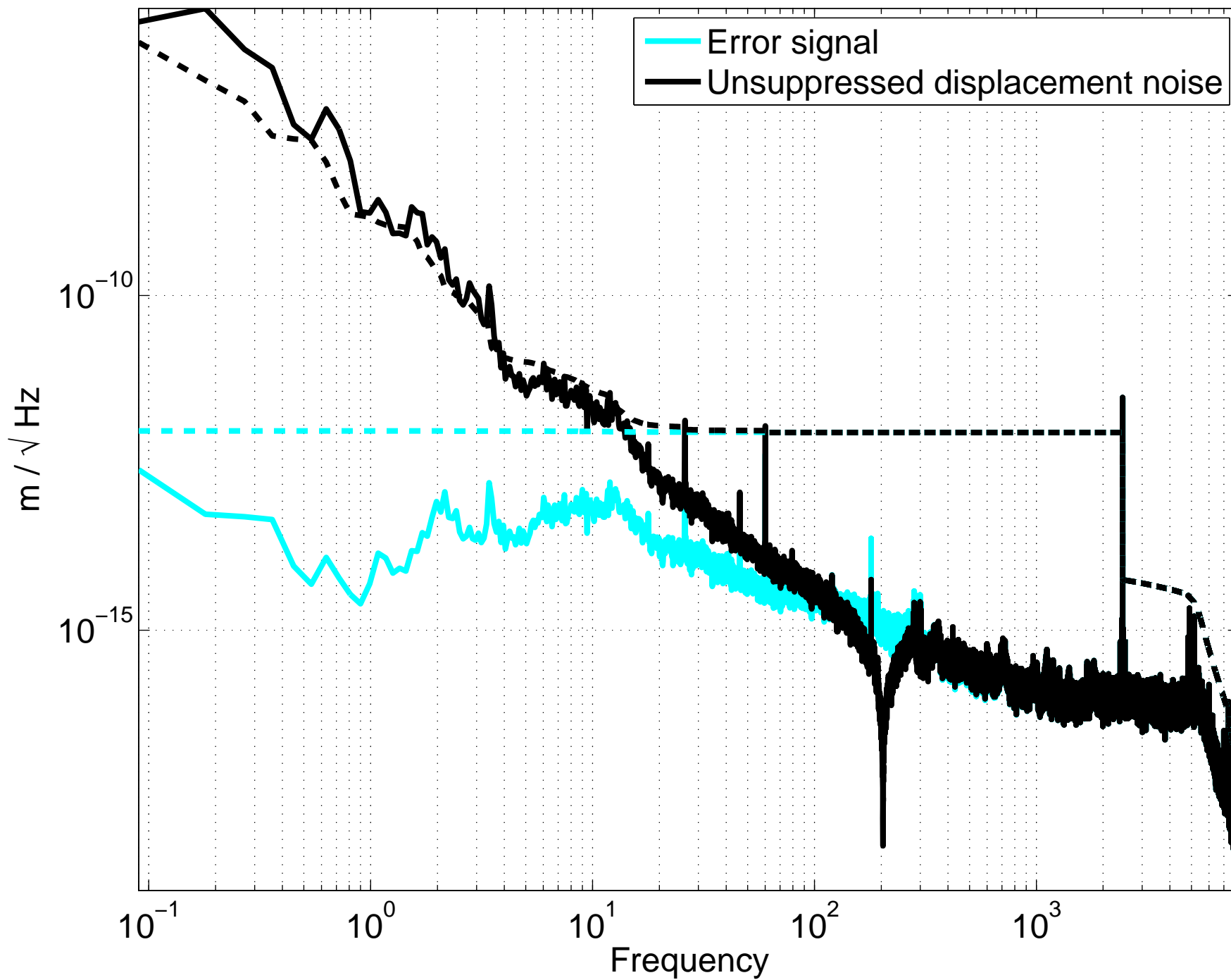
Calibrated PRCL signals
