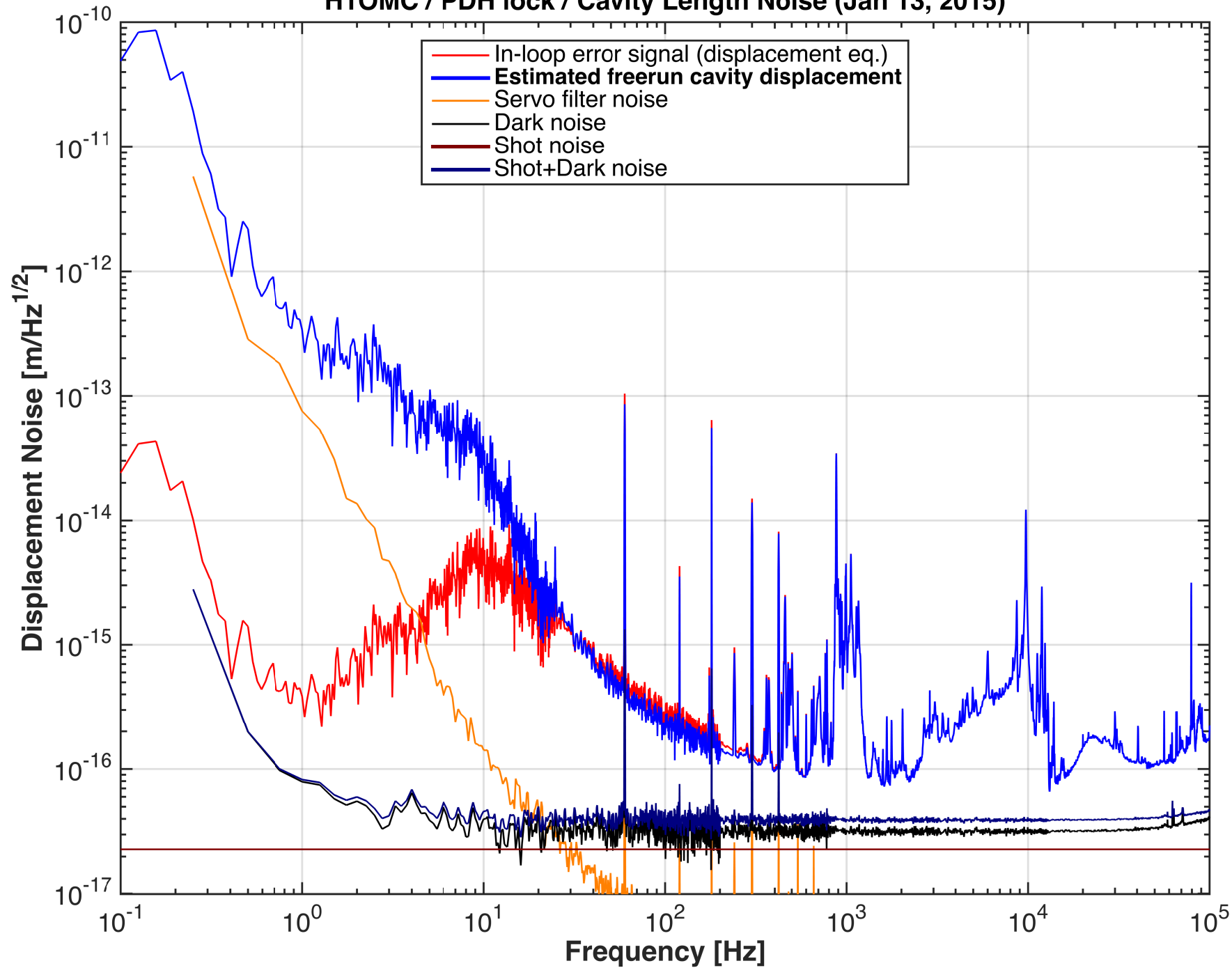
H10MC / PDH lock / Cavity Length Noise (Jan 13, 2015)
