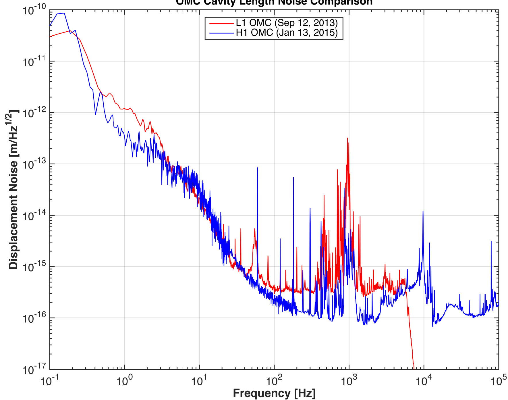
OMC Cavity Length Noise Comparison
