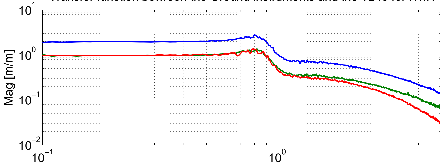
Transfer function between the Ground instruments and the T240 for ITMY
