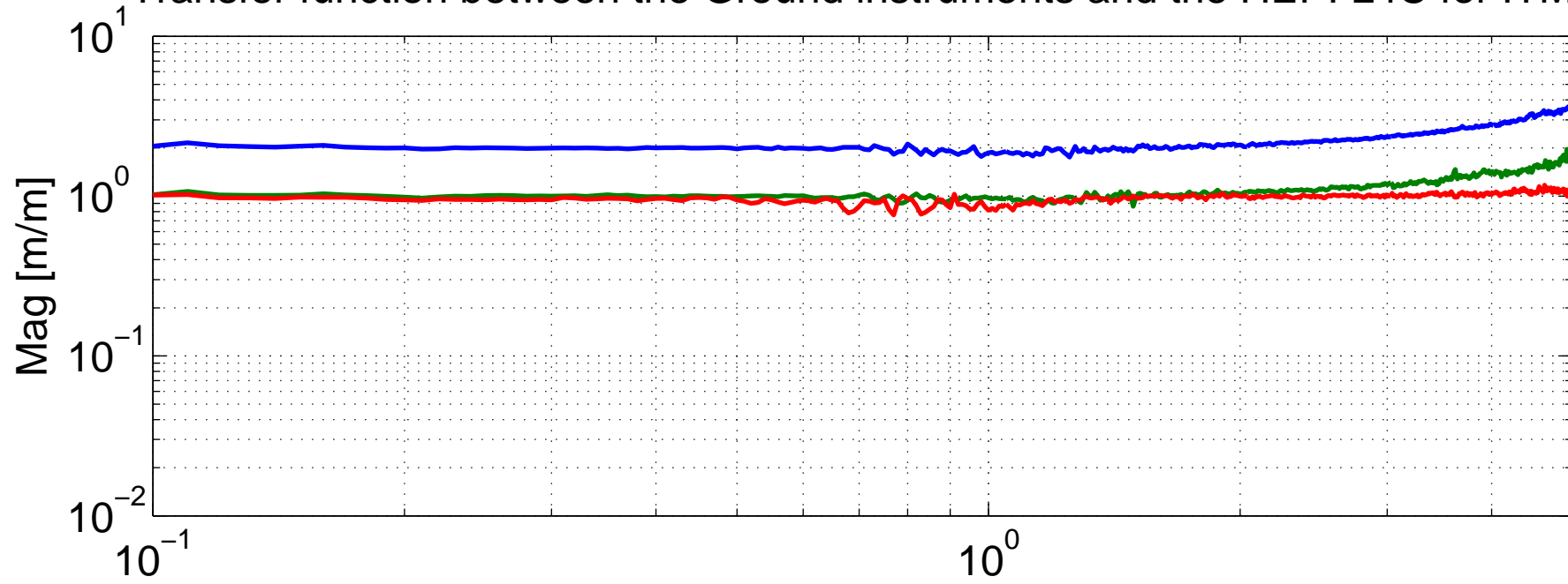
Transfer function between the Ground instruments and the HEPI L4C for ITMY
