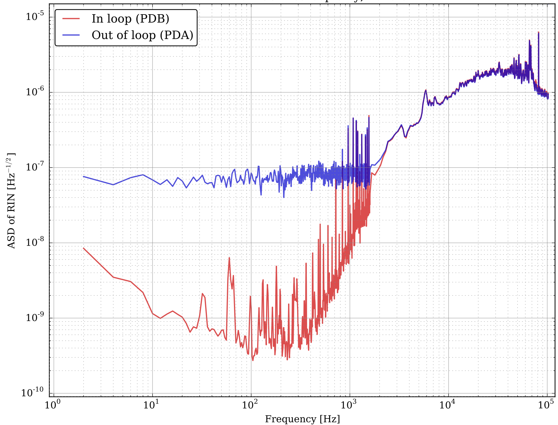
PSL RIN with ISS first loop only, 2015-01-23
