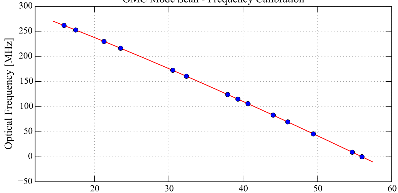
OMC Mode Scan - Frequency Calibration
