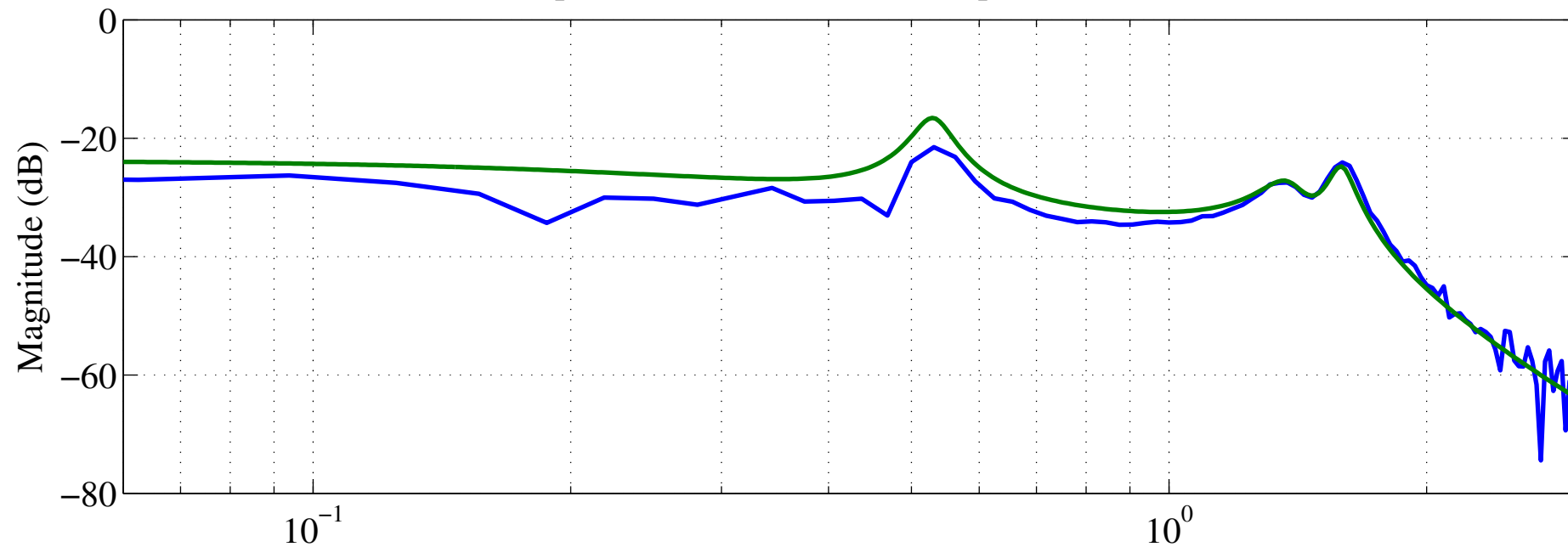
DHARD plant: ETMs' differential L2 pitch to AS45Q WFS
