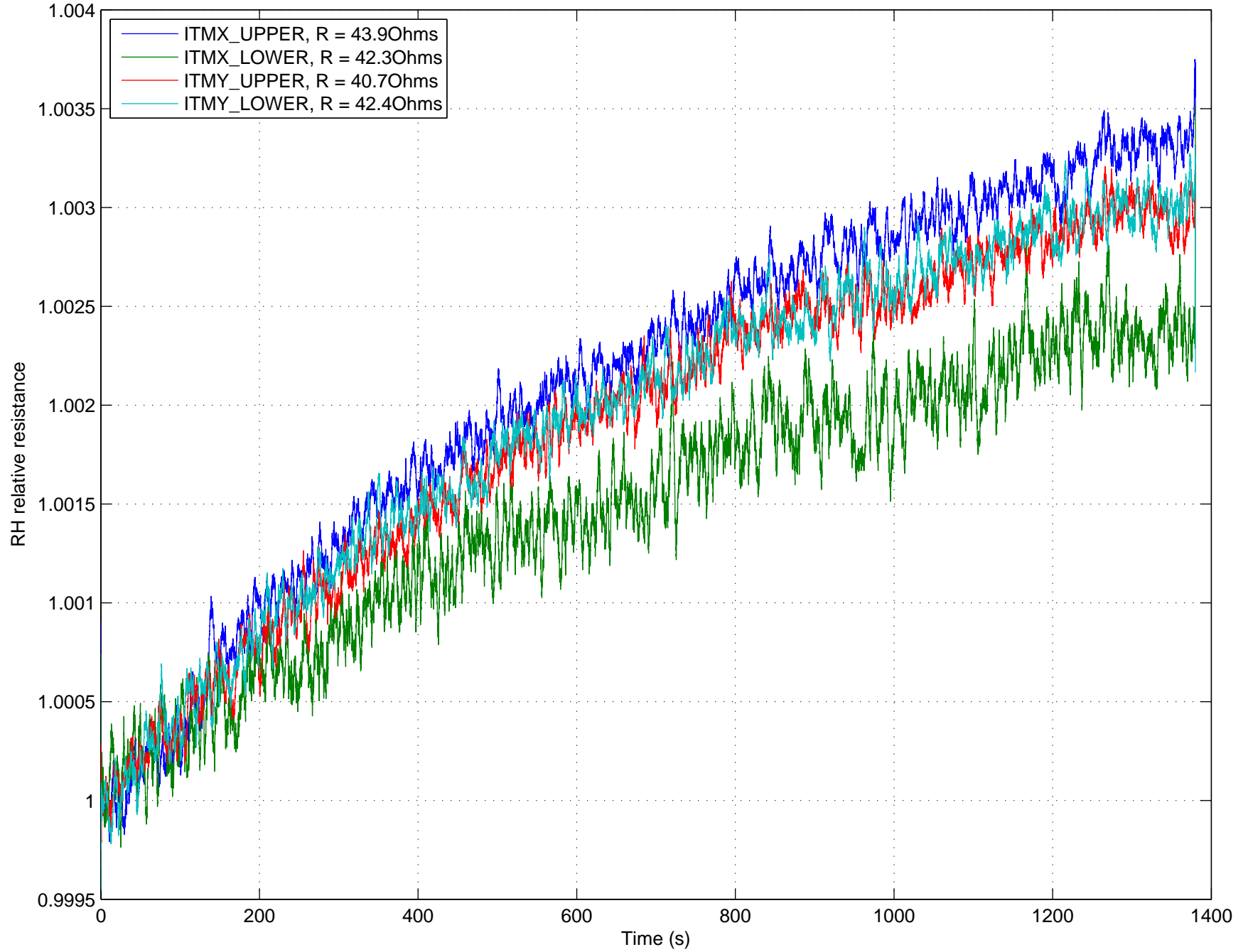
Relative increase in RH resistance vs time with 1W applied per segment
