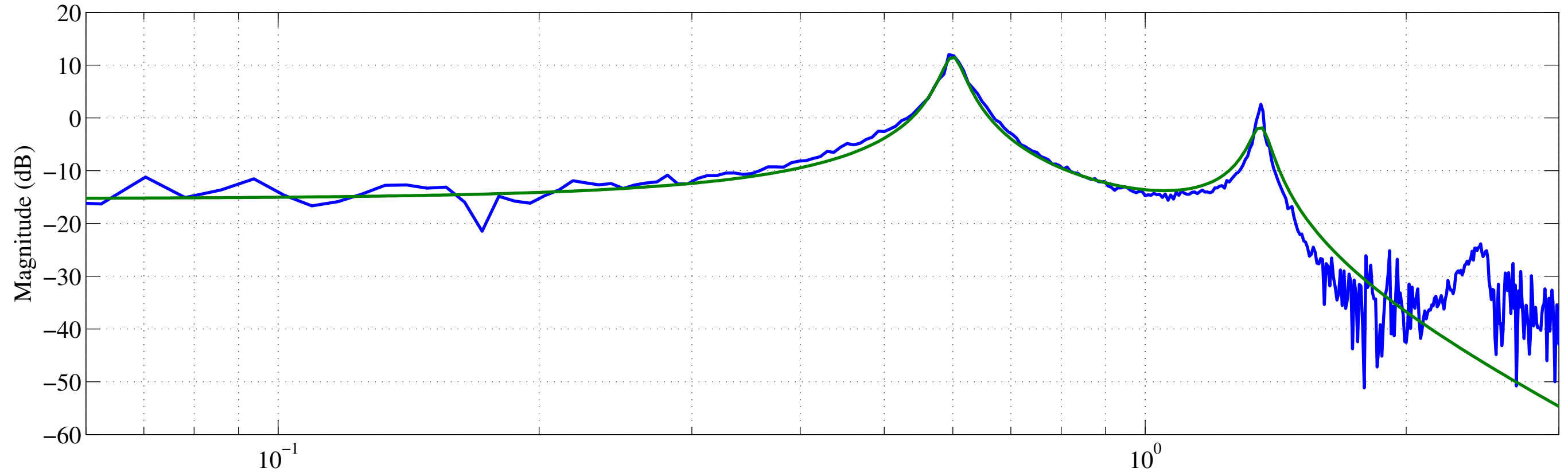
DHARD plant: ETMs' differential L2 yaw to AS45Q WFS
