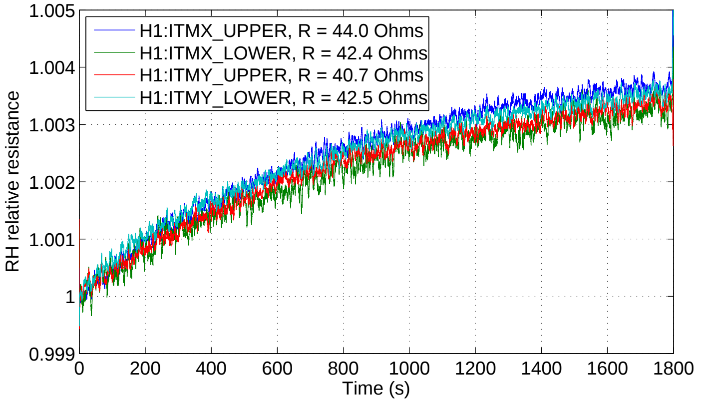
Relative increase in RH resistance vs time with 1W applied per segment
