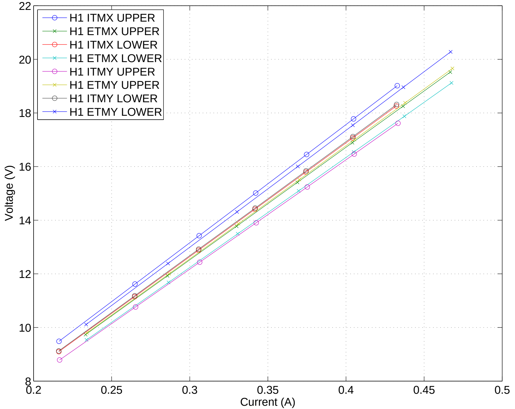
Current vs voltage for all RHs – slope = resistance
