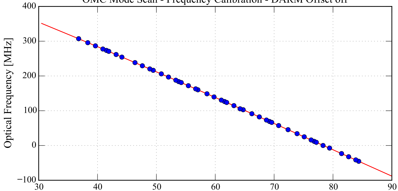
OMC Mode Scan - Frequency Calibration - DARM Offset off
