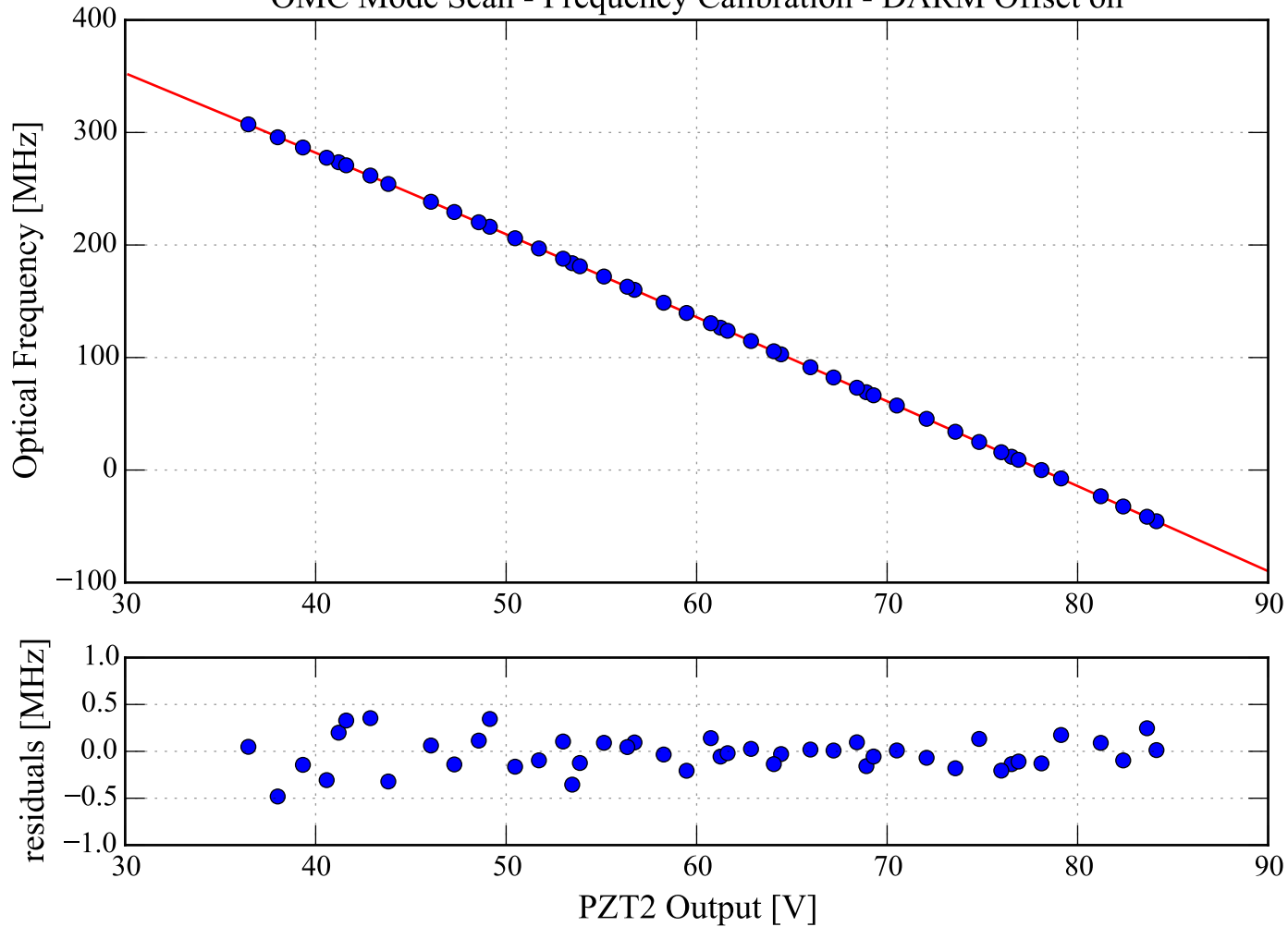
OMC Mode Scan - Frequency Calibration - DARM Offset on
