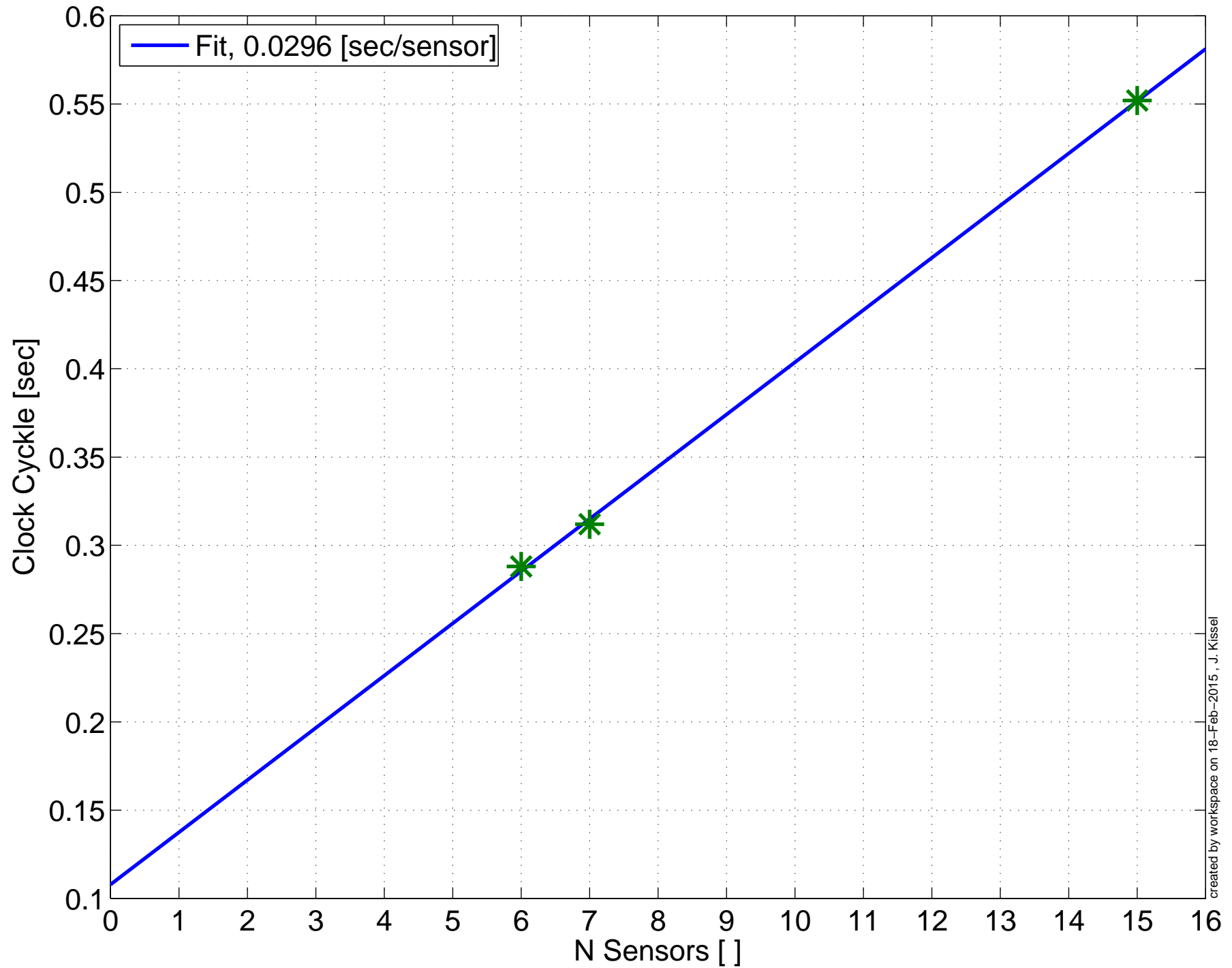
2015-02-18 HPI Pump Servo Computer Clock Cycle (or Sampling Rate) vs Number of Sensors
