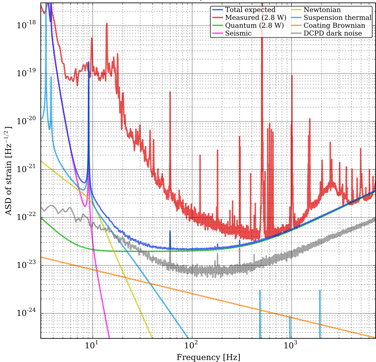
aLIGO H1 DARM strain, 2015-02-21 05:30:00 UTC
