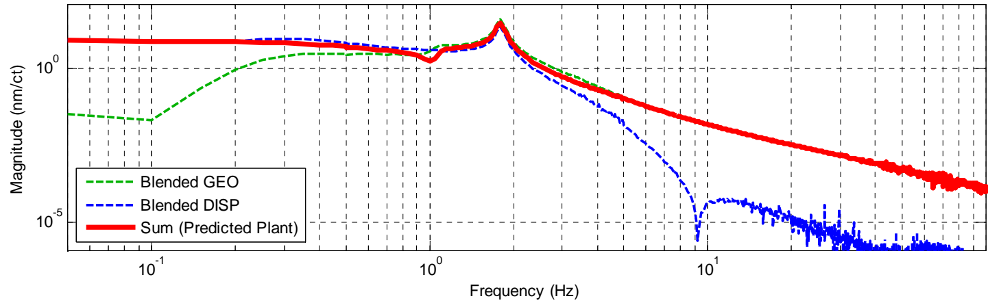
LHO HAM-ISI Unit 2 Aug 27, 2010 1 Hz Blend Filters Z Expected Blended Transfer Function
