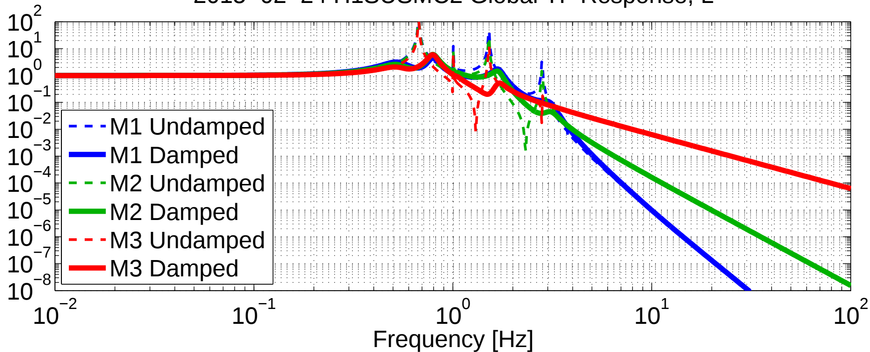
2015-02-24 H1SUSMC2 Global TF Response, L
