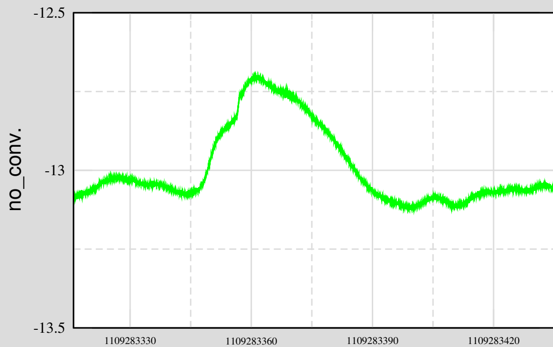
Ch 2: H1:SUS-BS_M3_OPLEV_YAW_OUT_DQ
