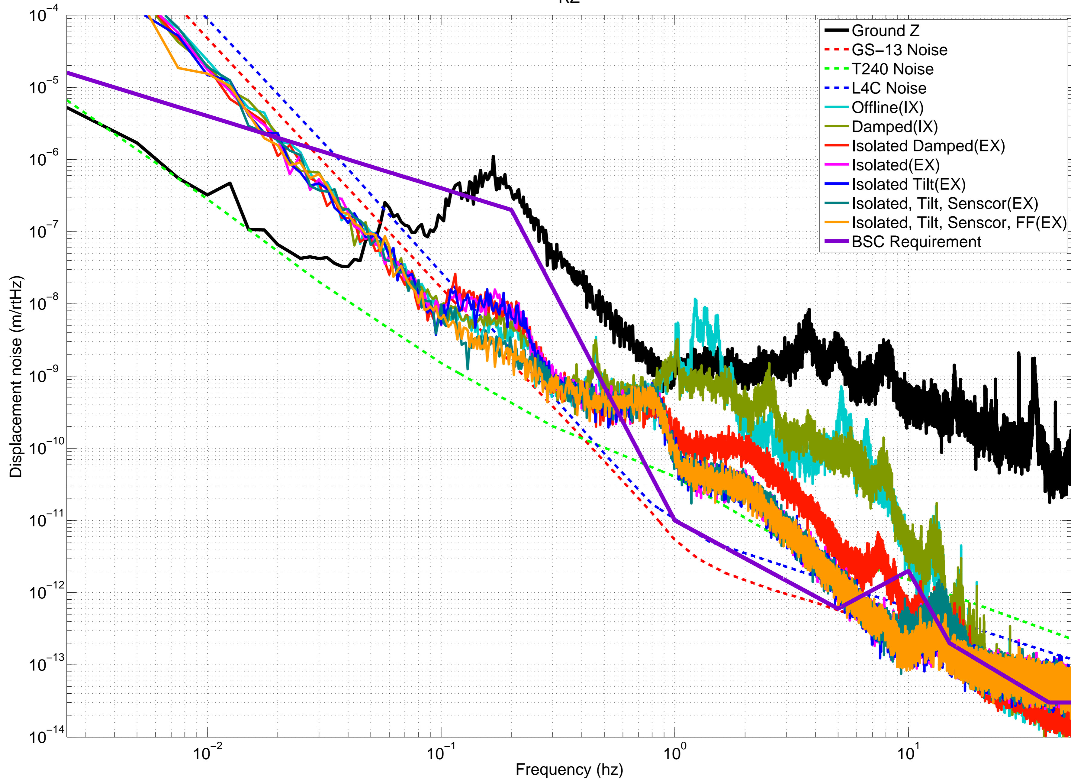
Control Contributions, St2 GS-13s RZ
