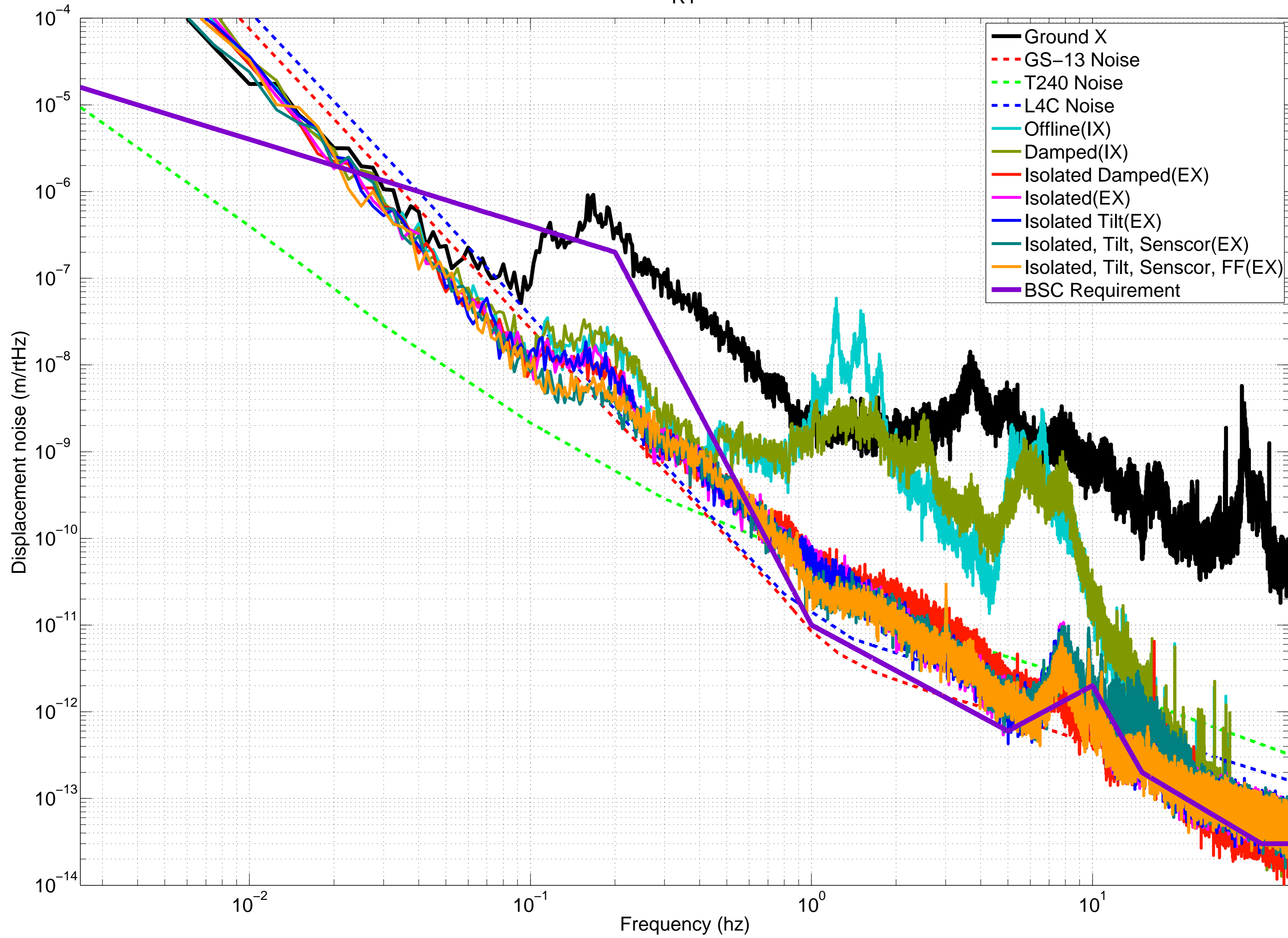
Control Contributions, St2 GS-13s RY
