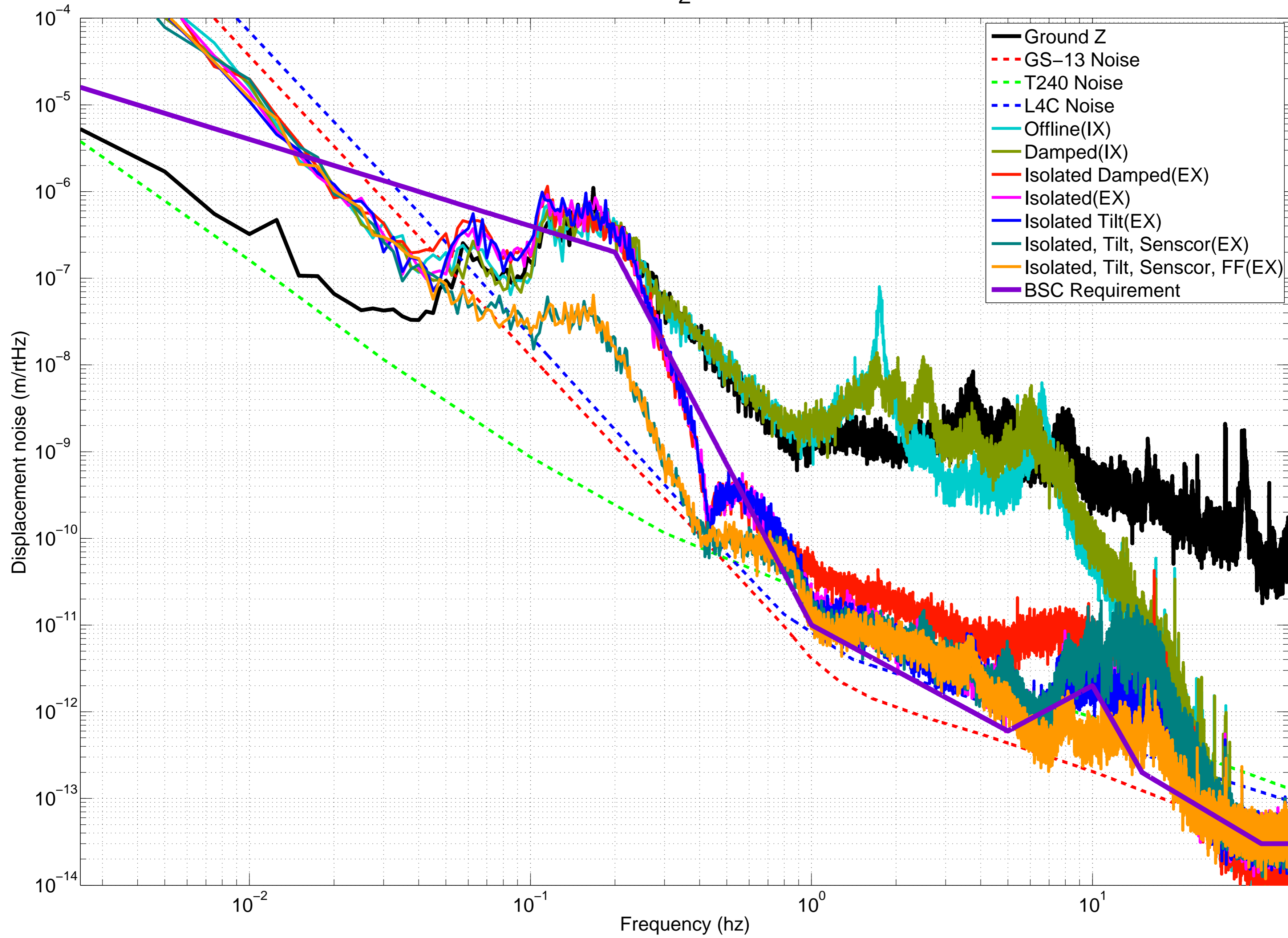
Control Contributions, St2 GS-13s Z
