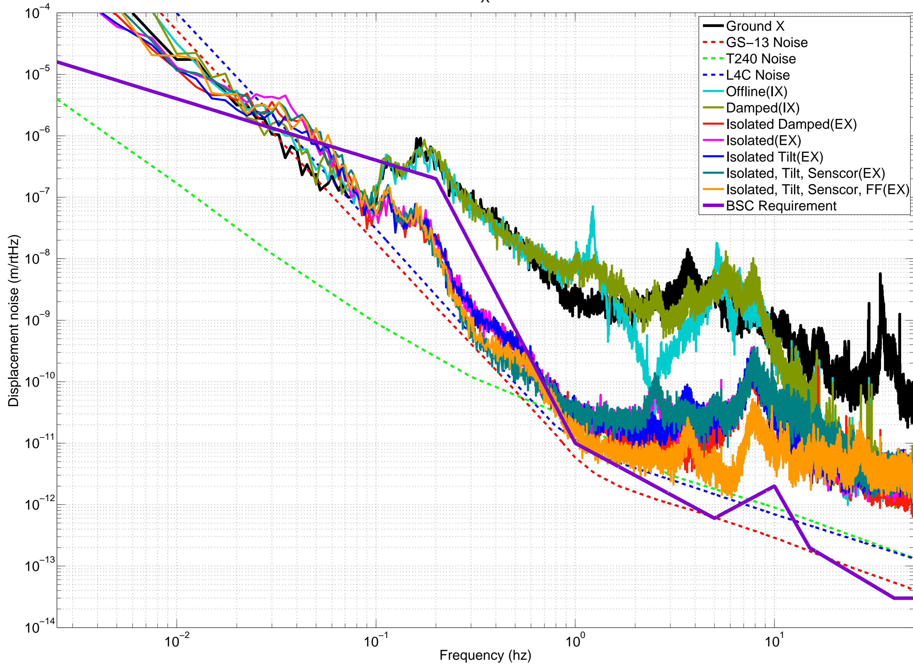
Control Contributions, St1 T240s X
