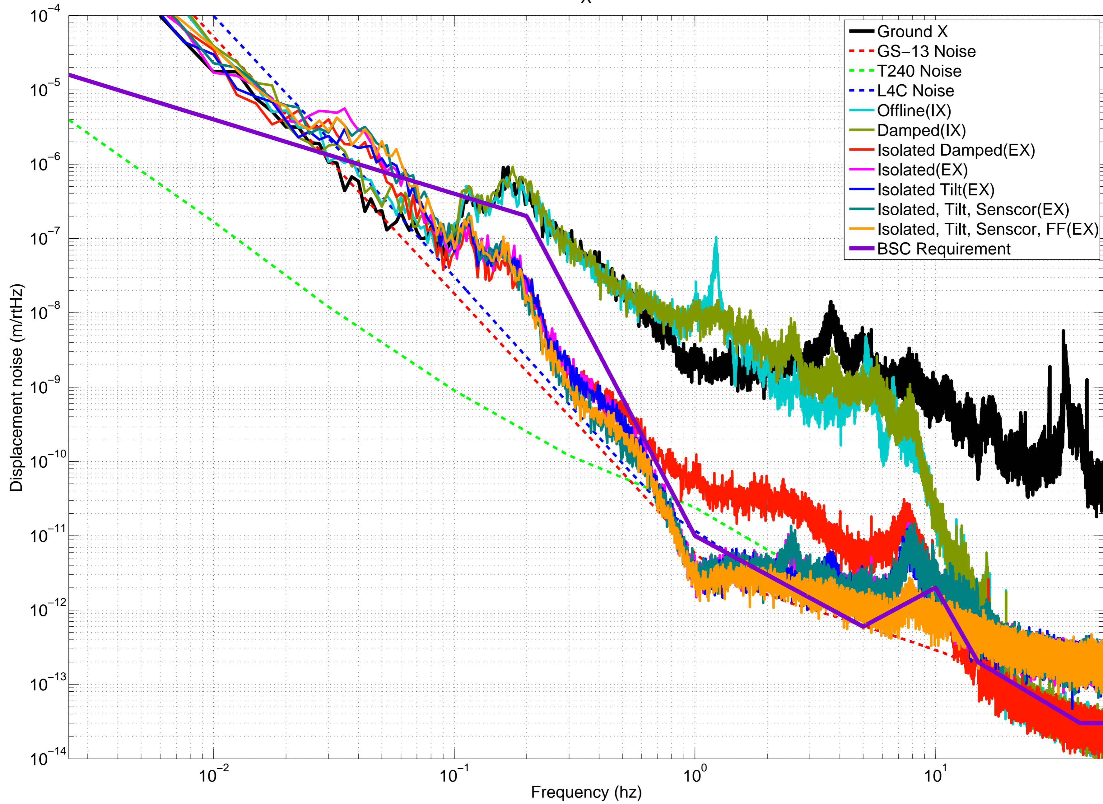
Control Contributions, St2 GS-13s X
